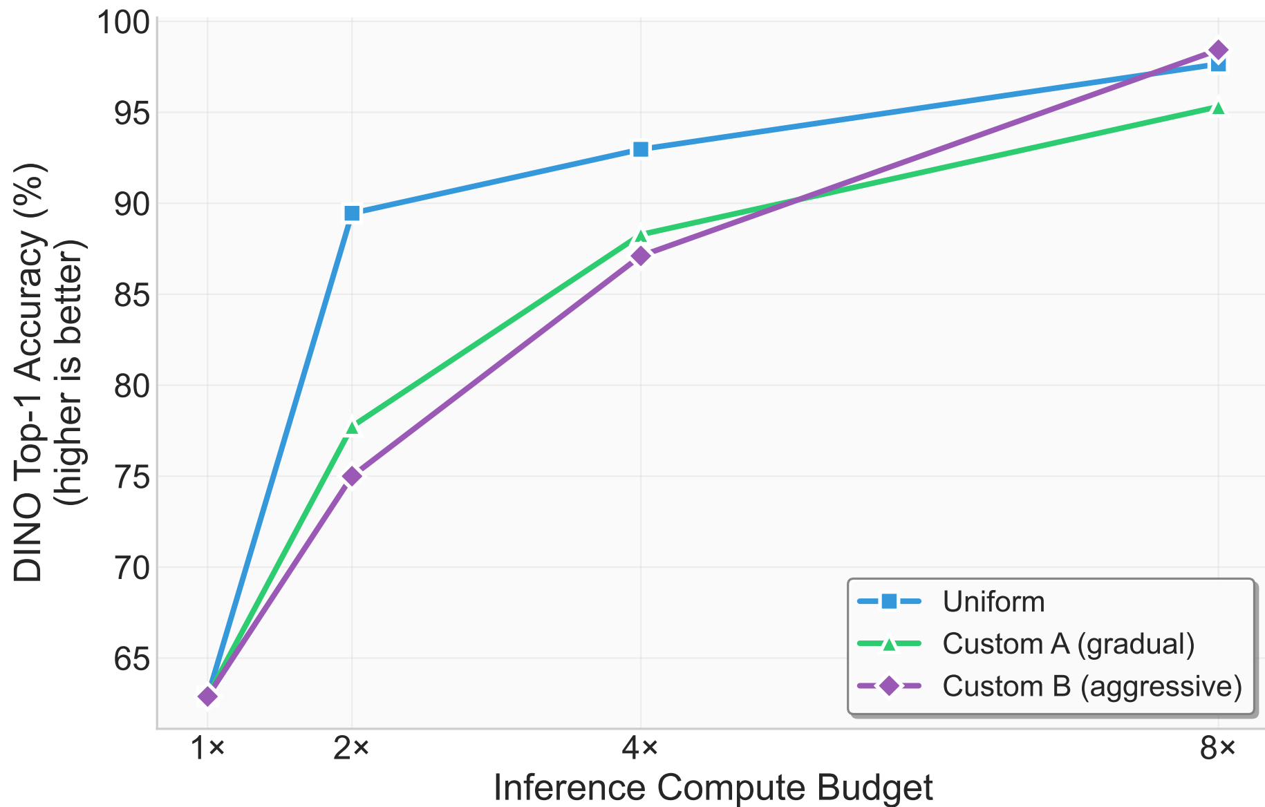
Non-Uniform Branching Ablation: DINO Top-1 Accuracy (%)
