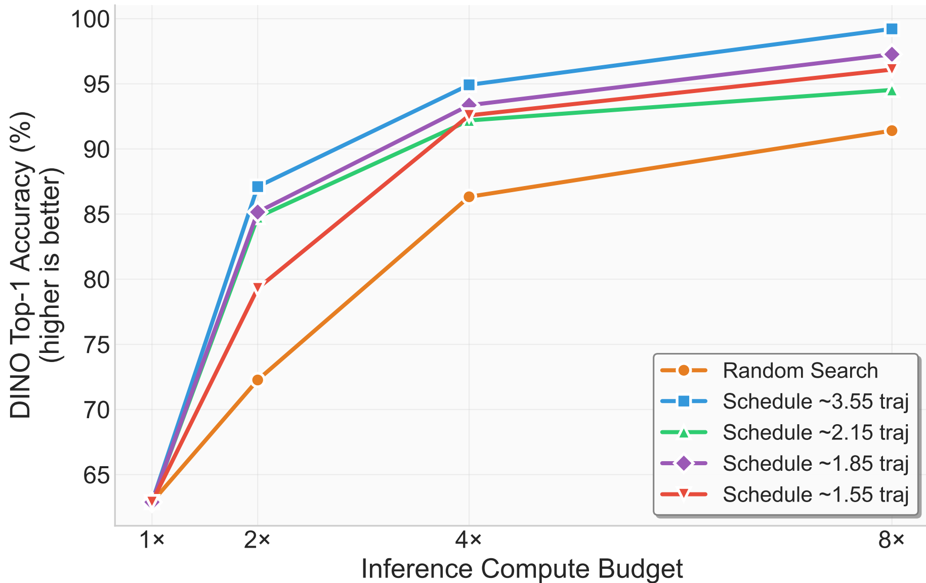
Branching Schedule Ablation: DINO Top-1 Accuracy (%)
