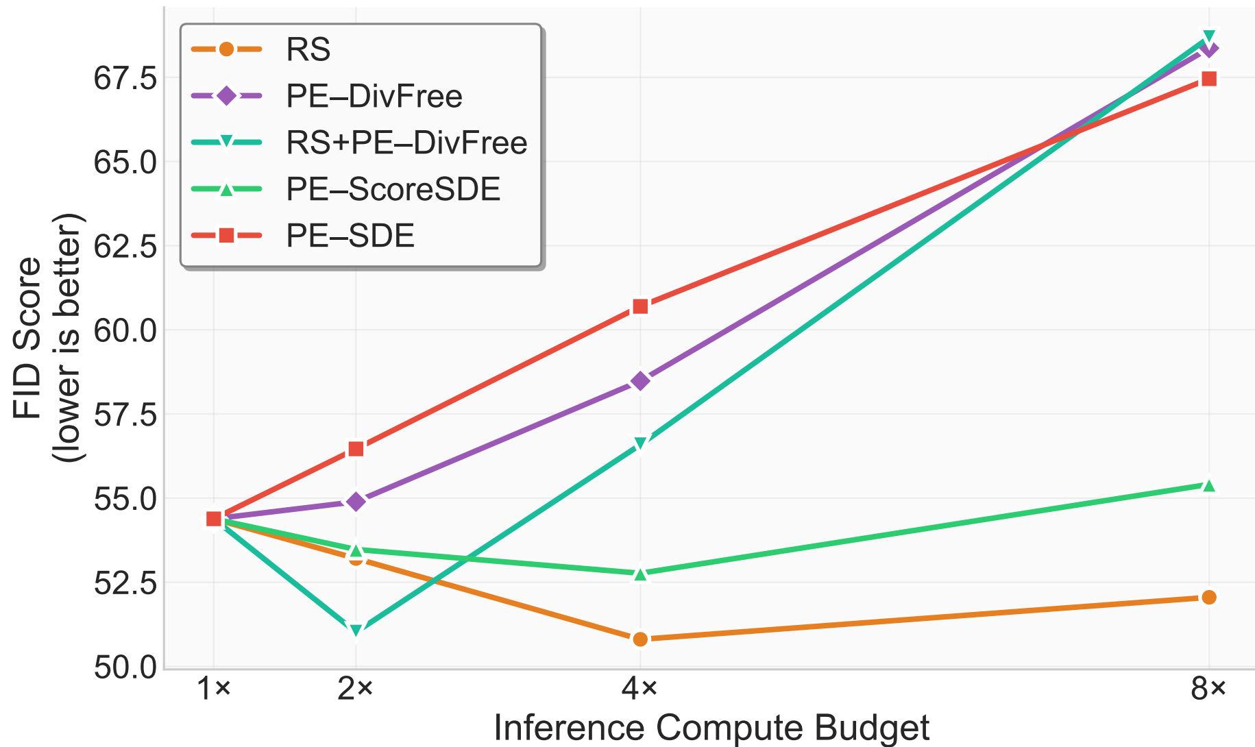
FID Score vs. Compute Budget Inception Verifier
