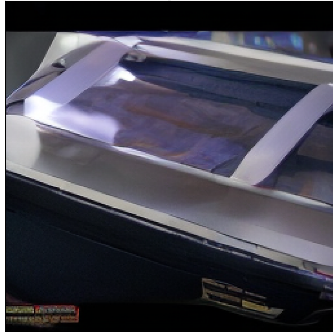
2x Computation
