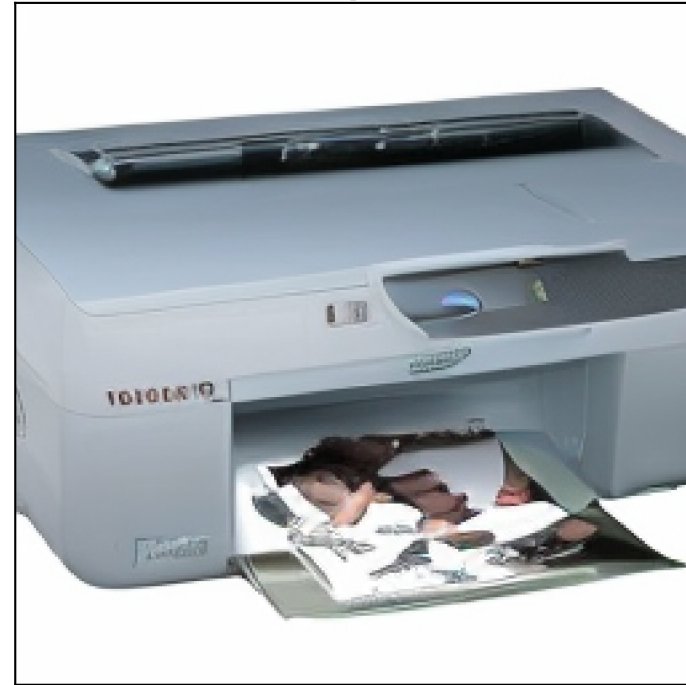
8x Computation
