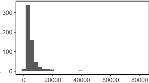
ApplicantIncome
