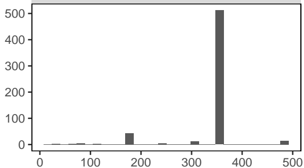
Loan_Amount_Term
