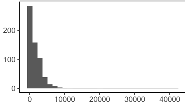
CoapplicantIncome
