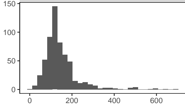
LoanAmount
