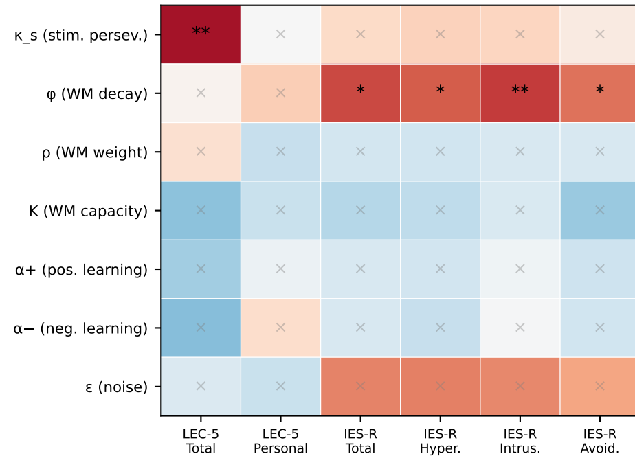
M6a: WM-RL + \kappa_s
