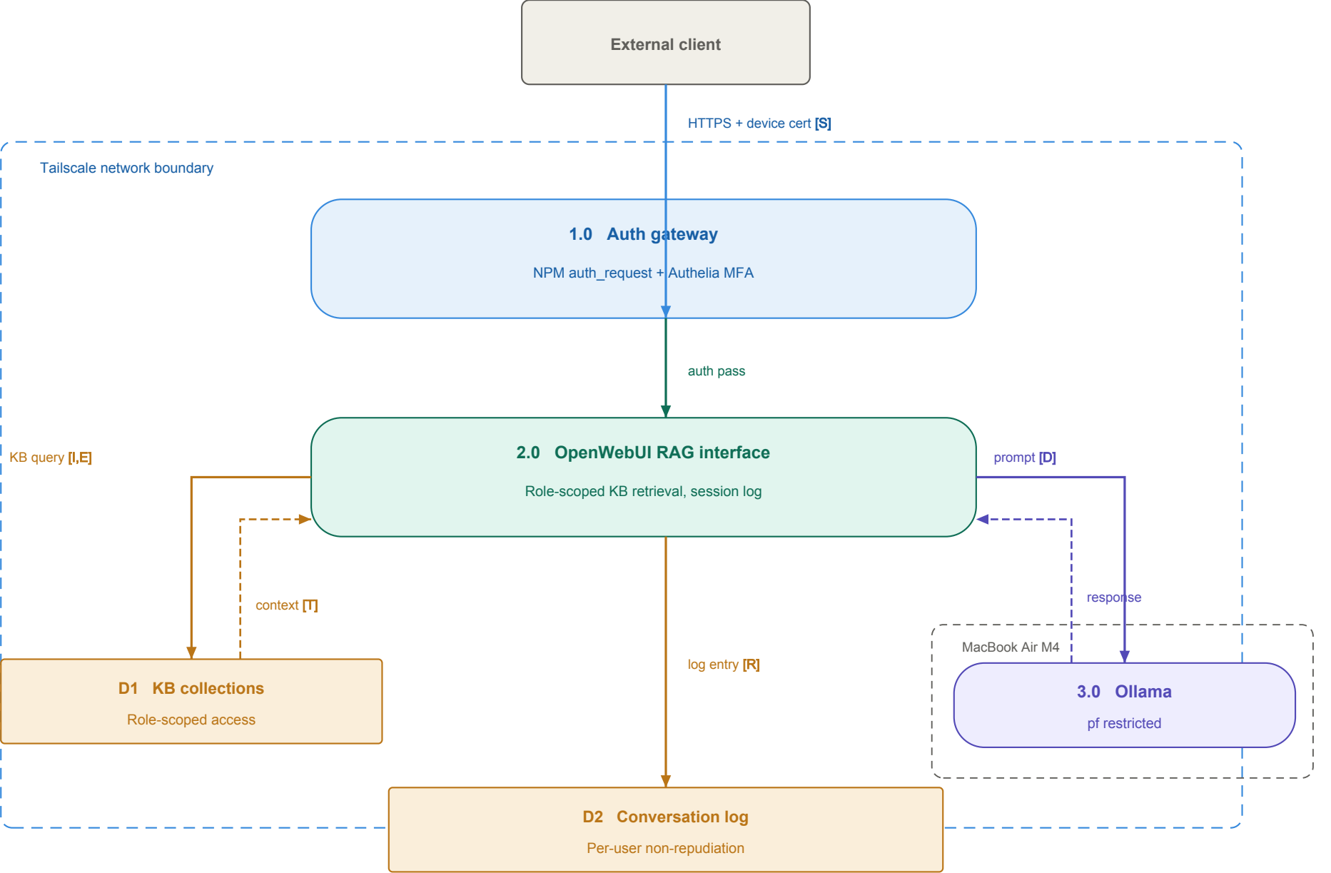
Level 1 Data Flow Diagram: RAG Pipeline
