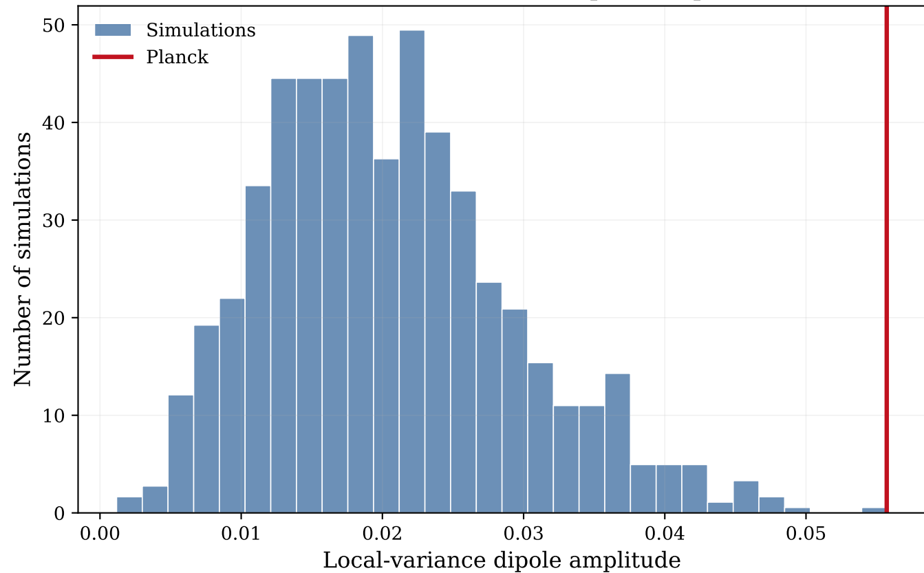
Fixed-scale local-variance dipole amplitude
