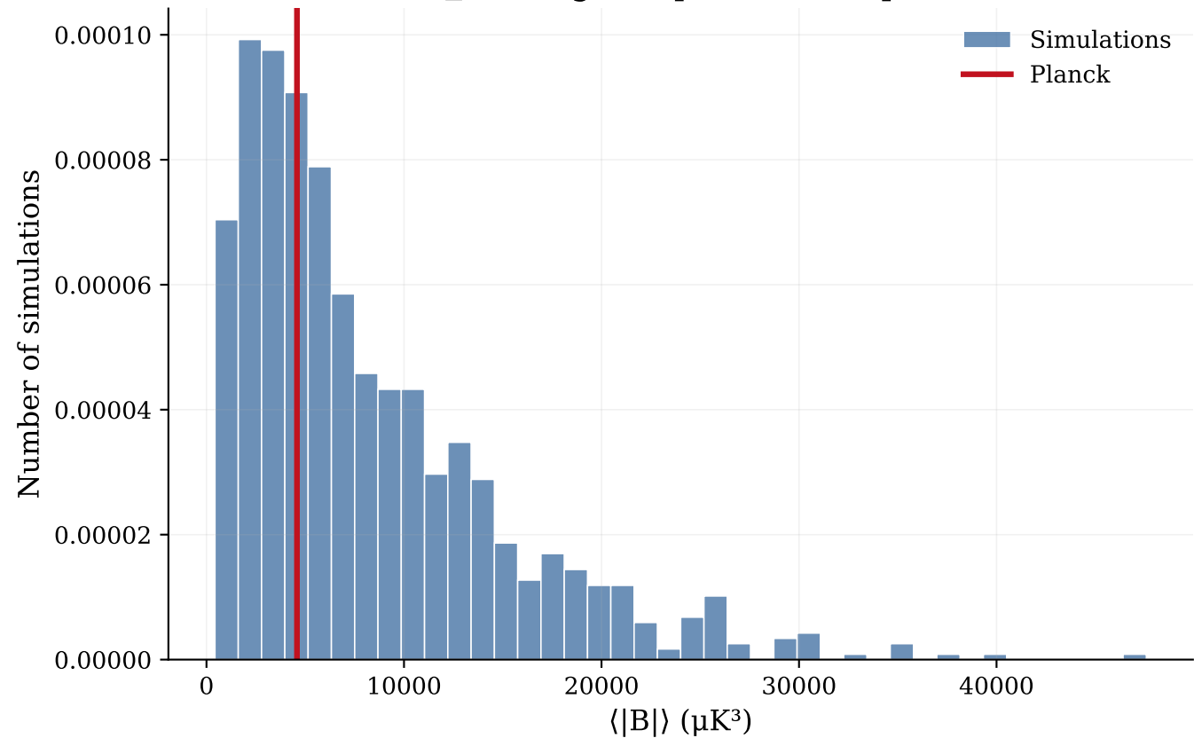
Low- \ell Average Bispectrum Amplitude
