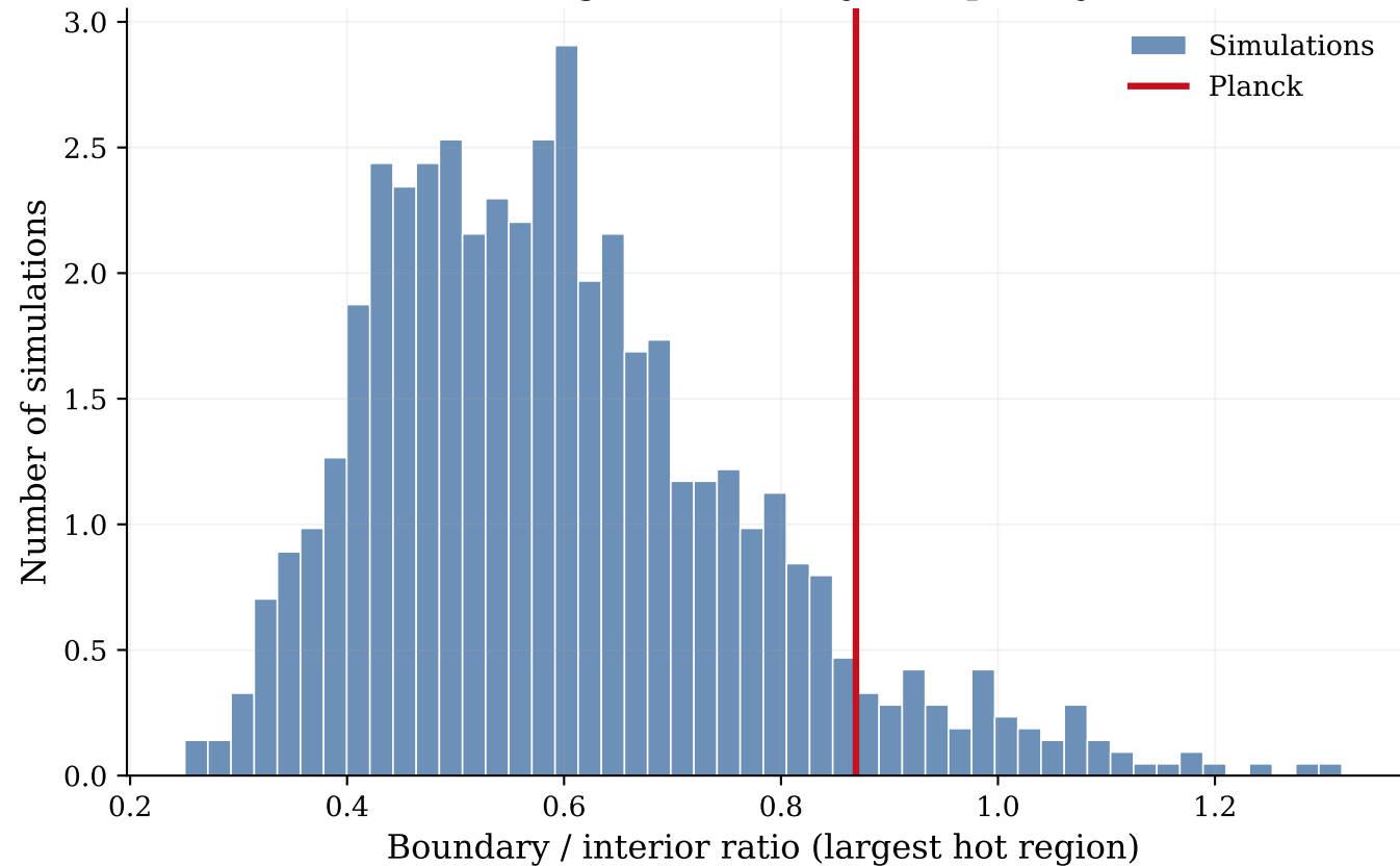
Low- \chi^2 Hot-Region Boundary Complexity Index
