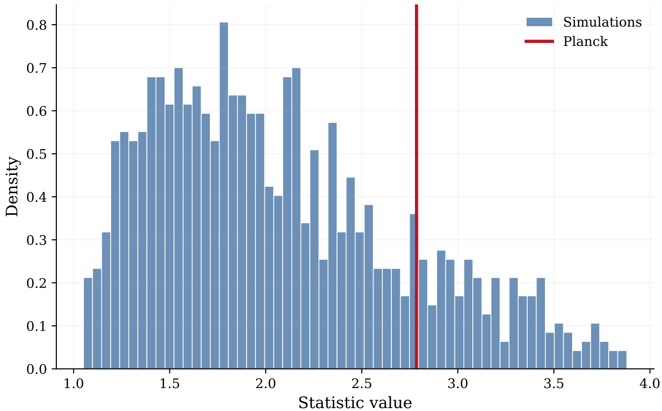
Simulation distribution vs Planck
