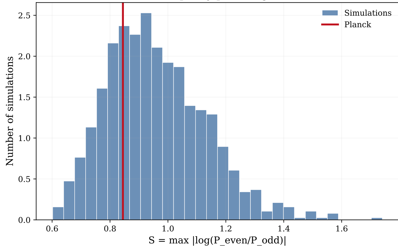
Low- l mirror-parity plane log-imbalance
