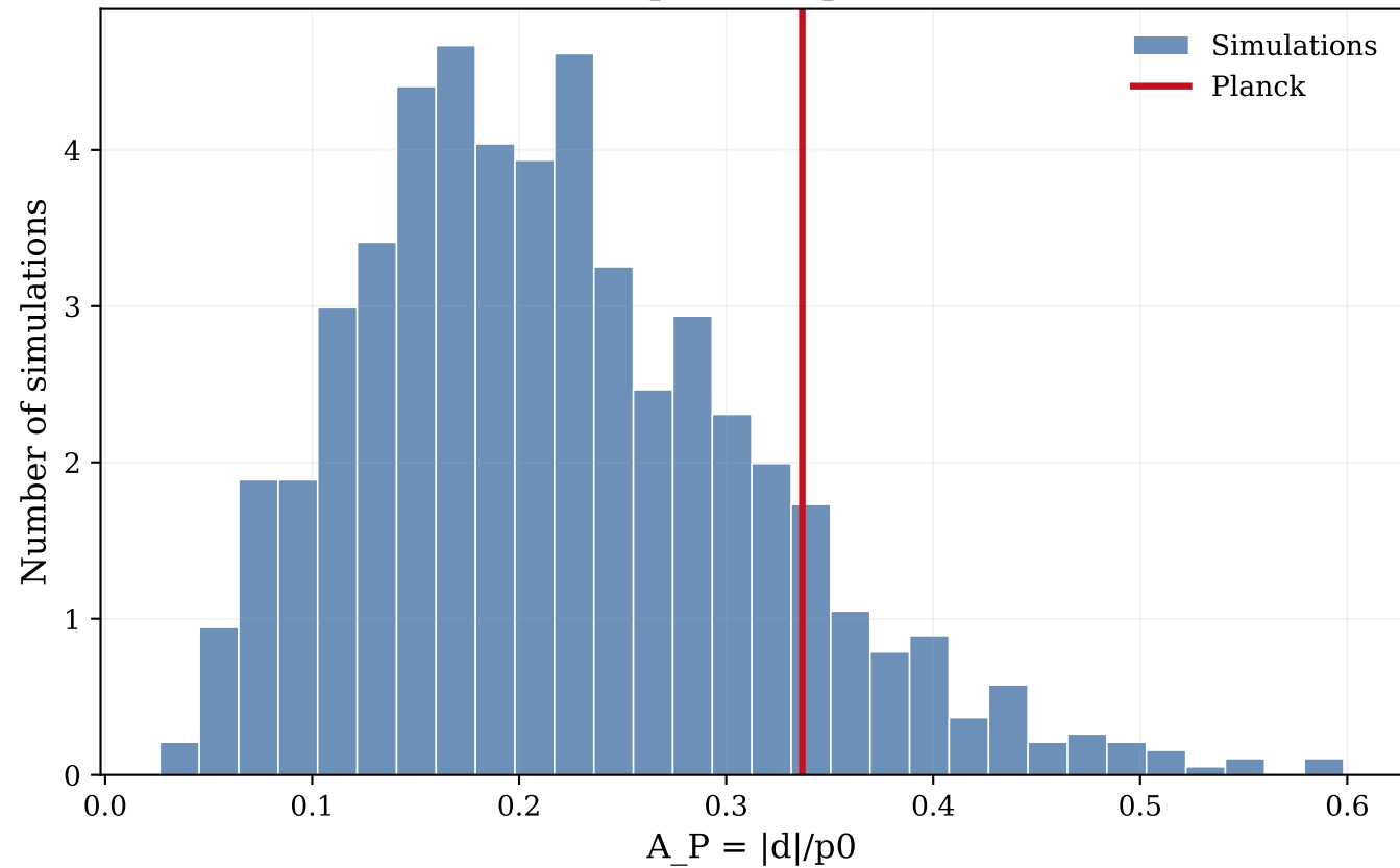
Low-l bandpower dipole fraction
