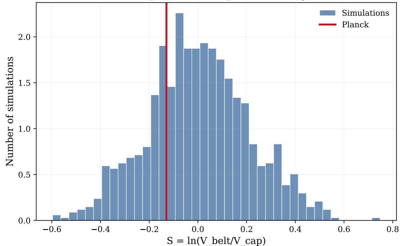
Low- l ecliptic belt-to-cap variance log-ratio
