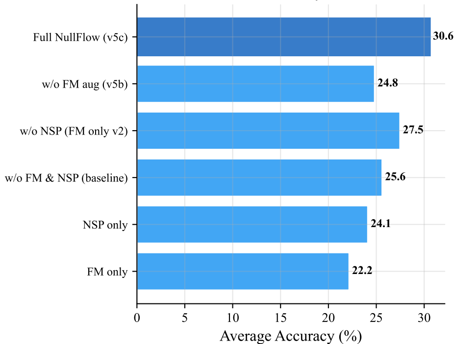
Accuracy
