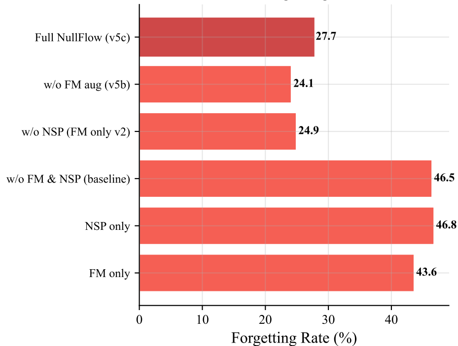
Forgetting
