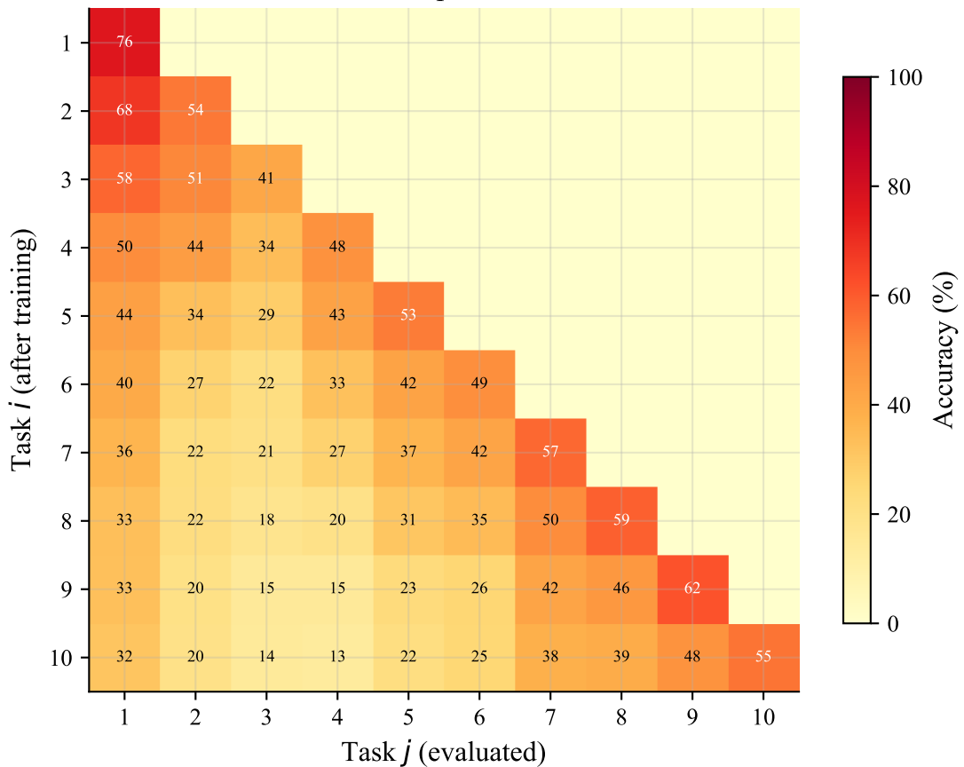
NullFlow — Split-CIFAR-100
