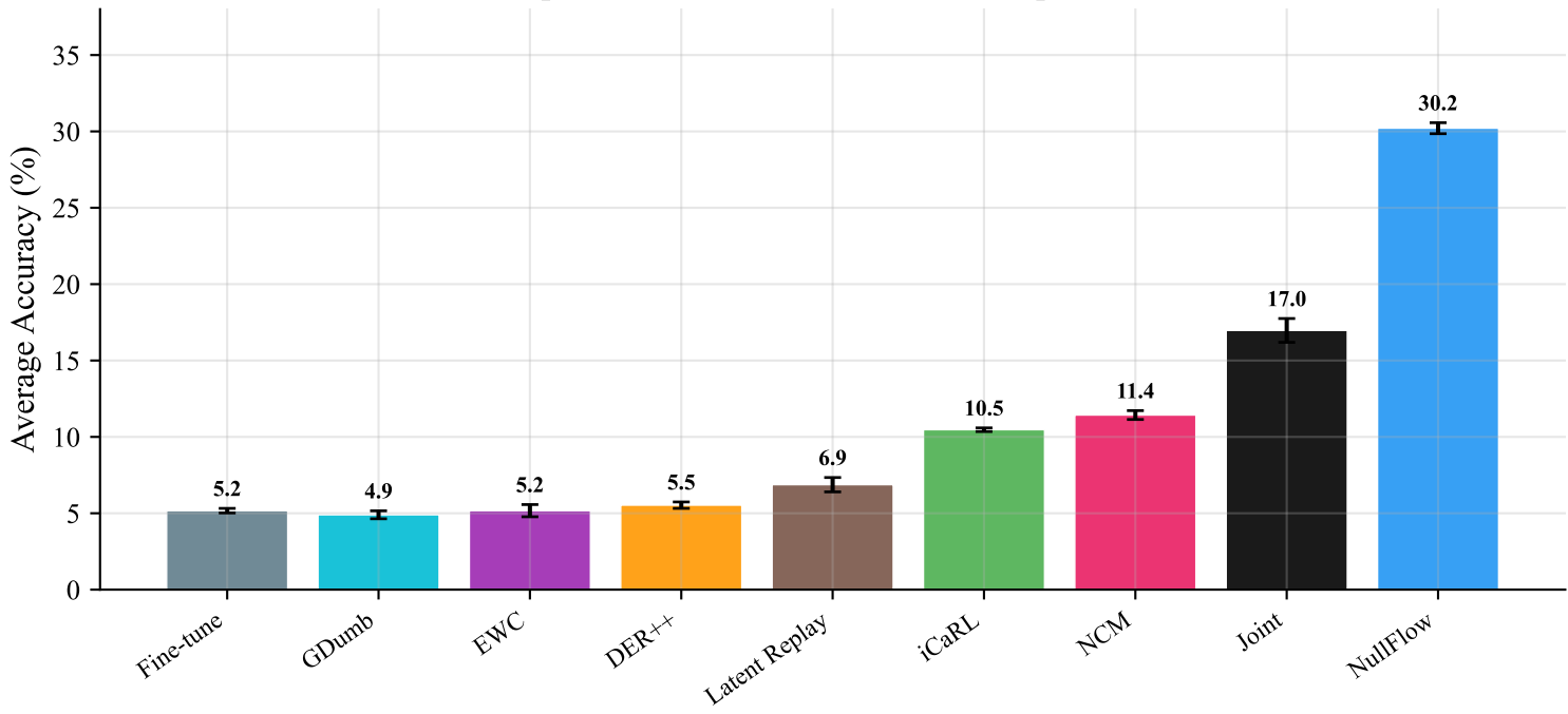
Split-CIFAR-100 — Baseline Comparison
