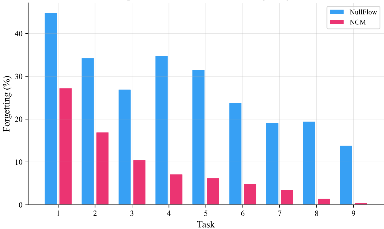
Split-CIFAR-100 — Per-Task Forgetting
