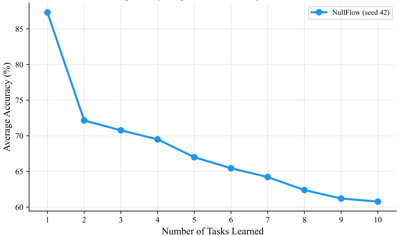
Split-TinyImageNet — Accuracy Evolution
