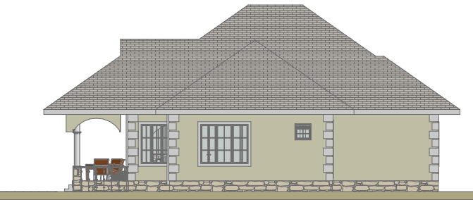
East Elevation (2)
