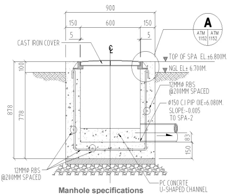
Manhole specifications
