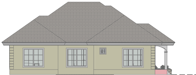
North Elevation (1) 1:100
