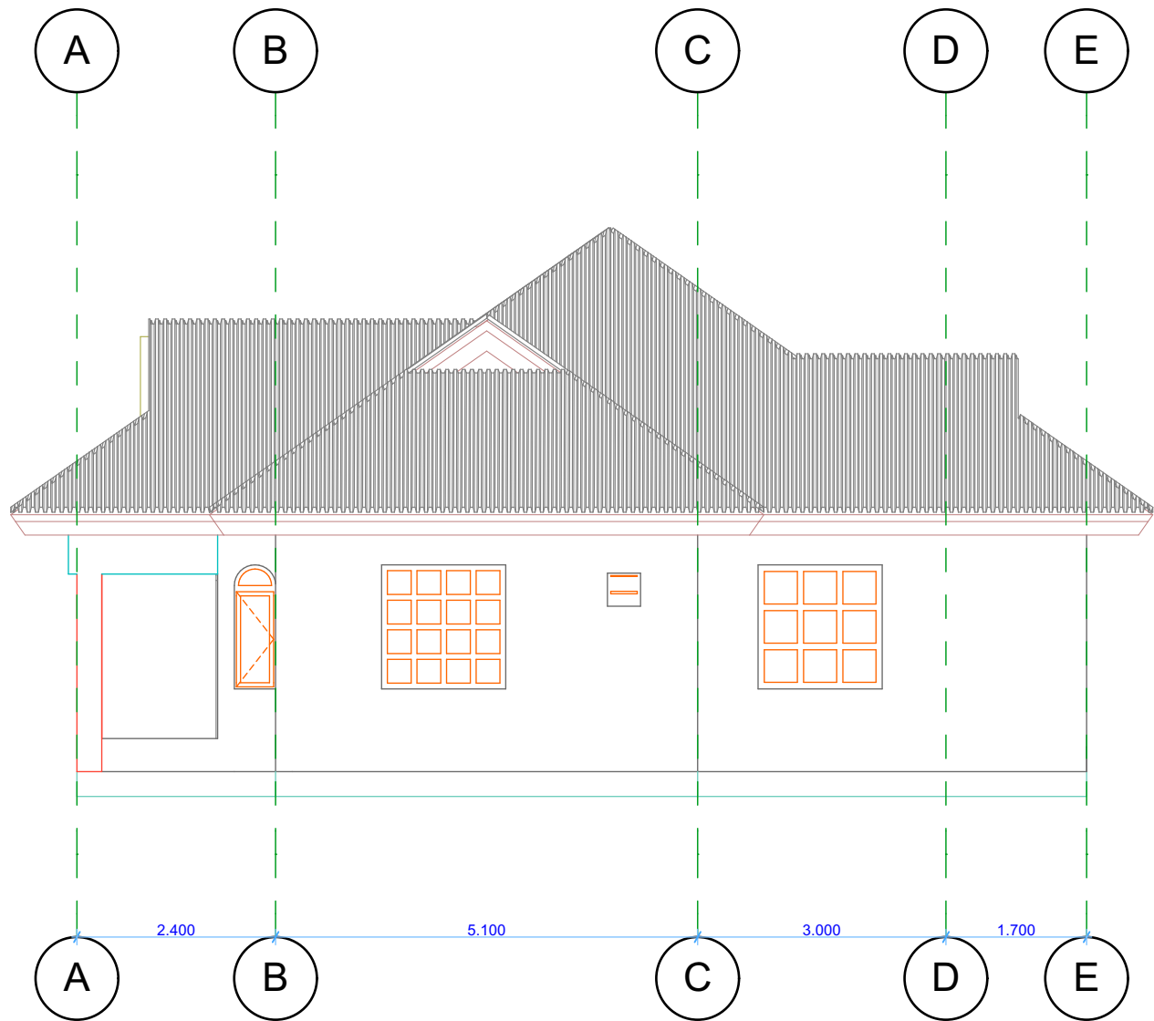
SIDE ELEVATION
