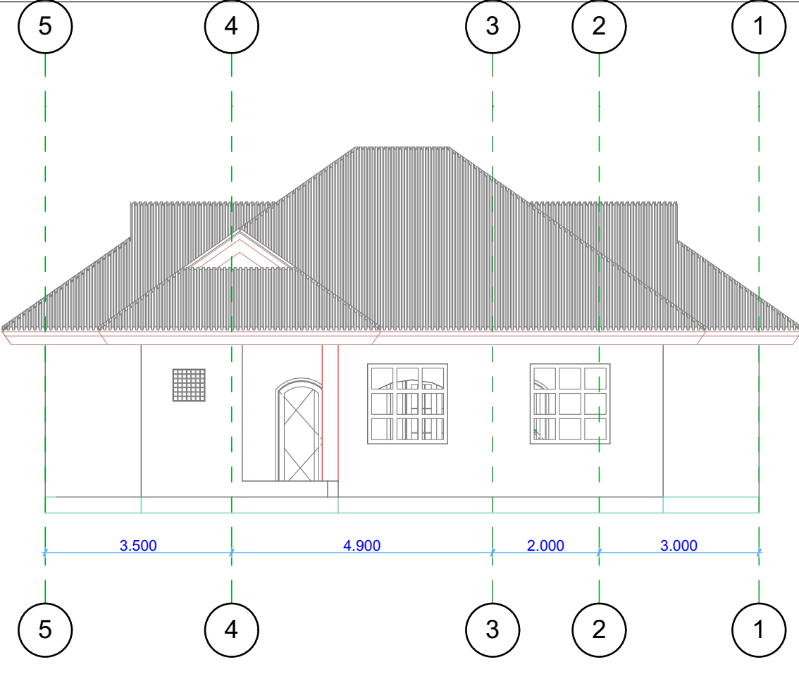
REAR ELEVATION
