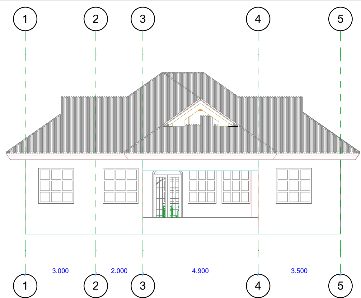
FRONT ELEVATION
