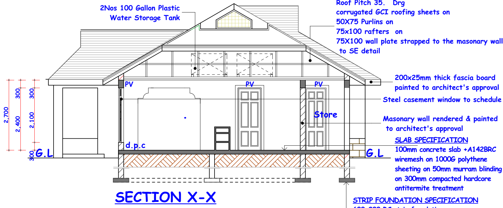
SECTION X-X
