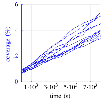
Fig. 3: Evolution of coverage over time for different history windows. Larger history windows result in slower initial coverage due to the increased influence of past trajectory data but lead to more stable long-term coverage. Over time, the differences diminish as all configurations converge toward their respective steady-state behaviors.
