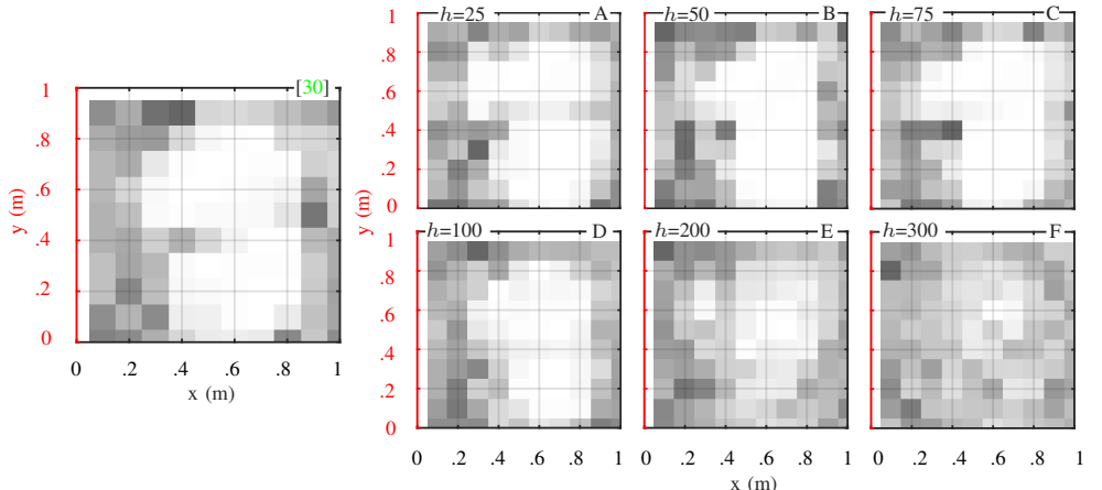
Fig. 6: Comparative results between the adaptive ergodic controller and the ergodic controller from [30]. The left-most figure replicates the coverage map from [30], where darker squares indicate areas of high information measure and lighter squares indicate areas of low information measure. The right-side figures illustrate the adaptive ergodic controller with different history windows A–F. The adaptive controller operates without an explicit underlying information measure, instead treating the original information distribution as two unknown obstacles that “are discovered upon proximity.”
