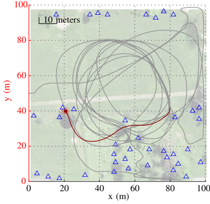
Fig. 5: Outdoor model of a large-scale vegetated area featuring our ergodic controller. The figure illustrates the UAV's trajectory over a 10 000 square-meter area located in Birmensdorf, Switzerland. The area features dense vegetation in an agricultural field. The dark red line represents the exploration history, while the dark red dot marks the UAV's current position. The problem is posed so that the modeled UAV operates at an altitude of 2.5 meters, avoiding tree trunks but not smaller bushes. The dynamics are adjusted to reflect real-world conditions, with the exploration history set to 150 time steps.
