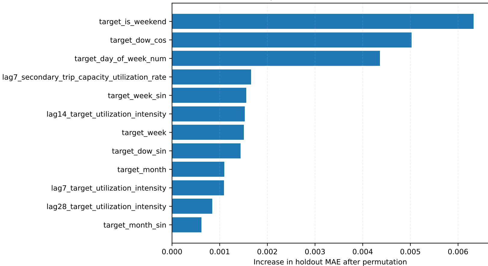
Post-hoc S2 random-forest permutation importance Synthetic demonstration data
