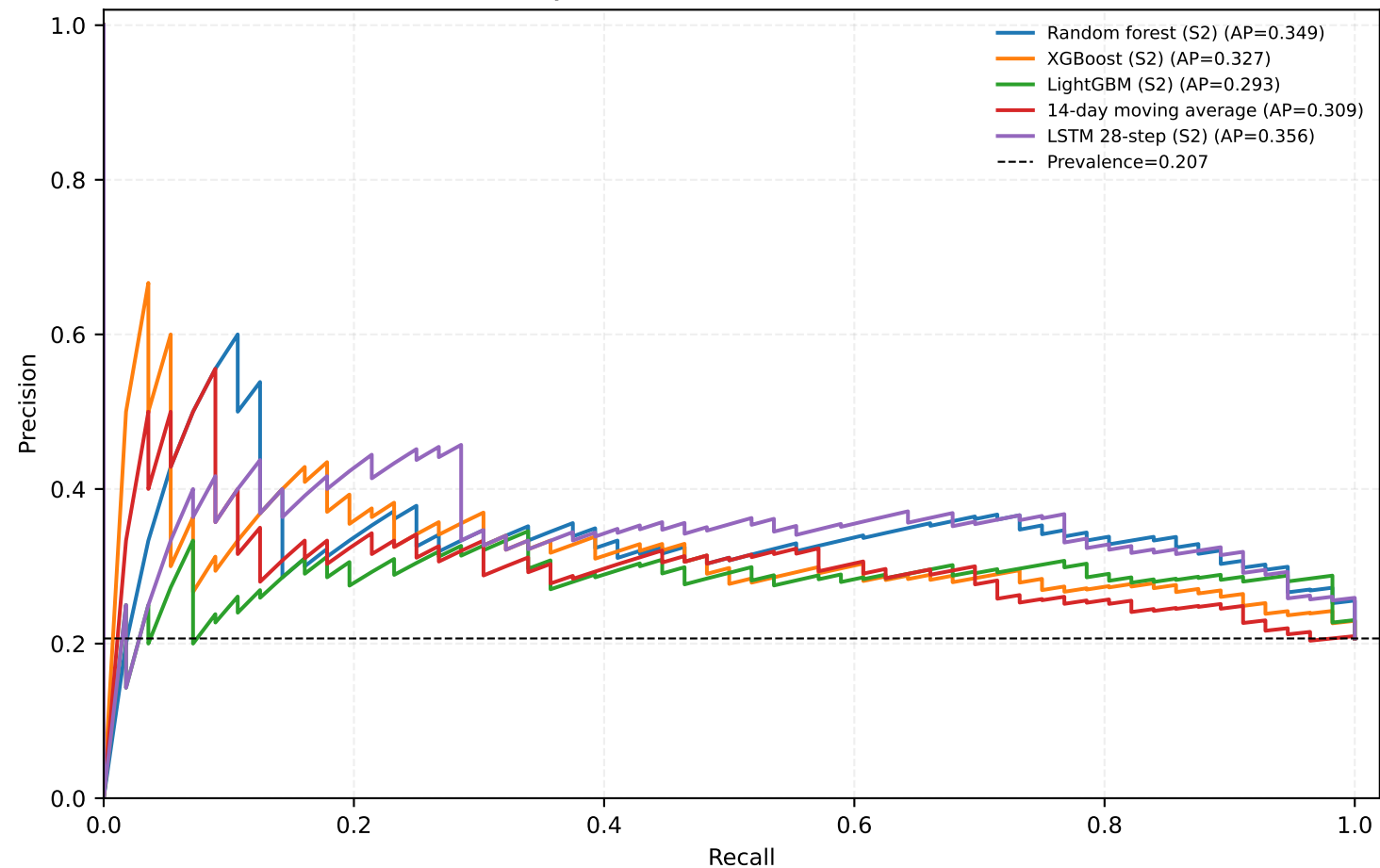
Stress-day precision-recall curves Synthetic demonstration data
