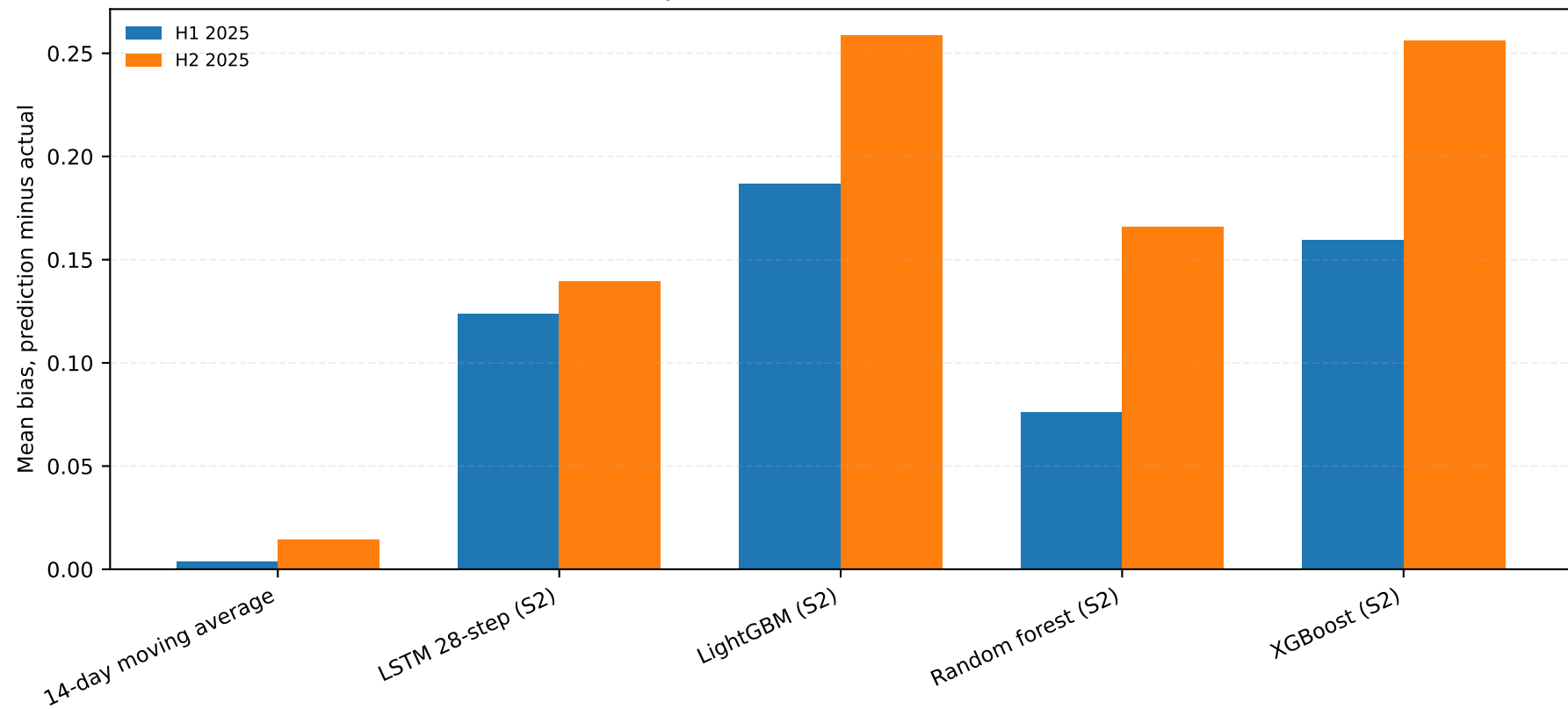
Prediction-bias shift by holdout regime Synthetic demonstration data
