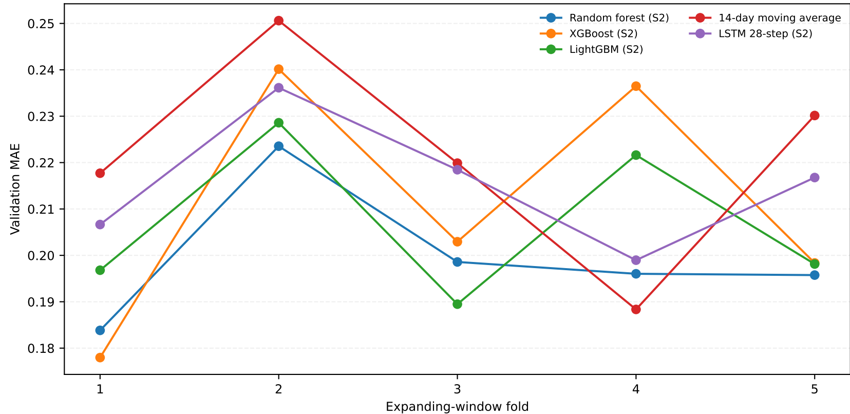
Fold-level MAE stability Synthetic demonstration data
