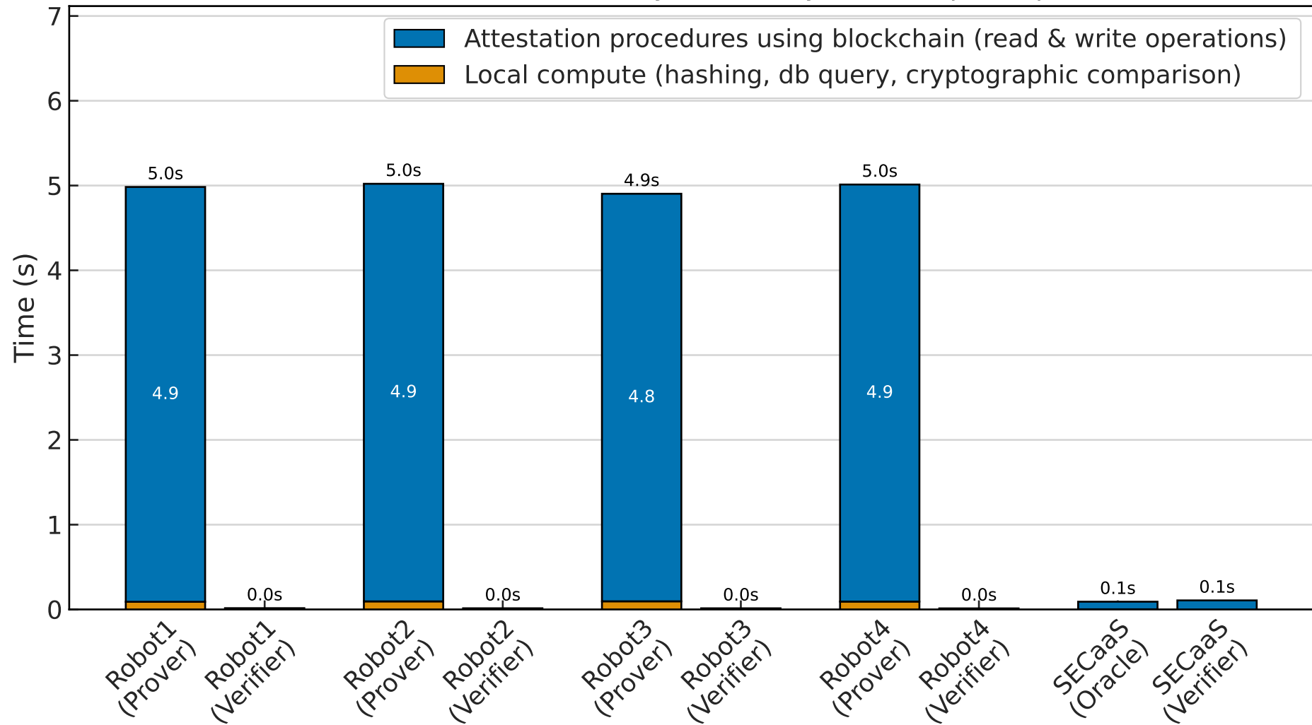
Breakdown of attestation cycle time by role and participant
