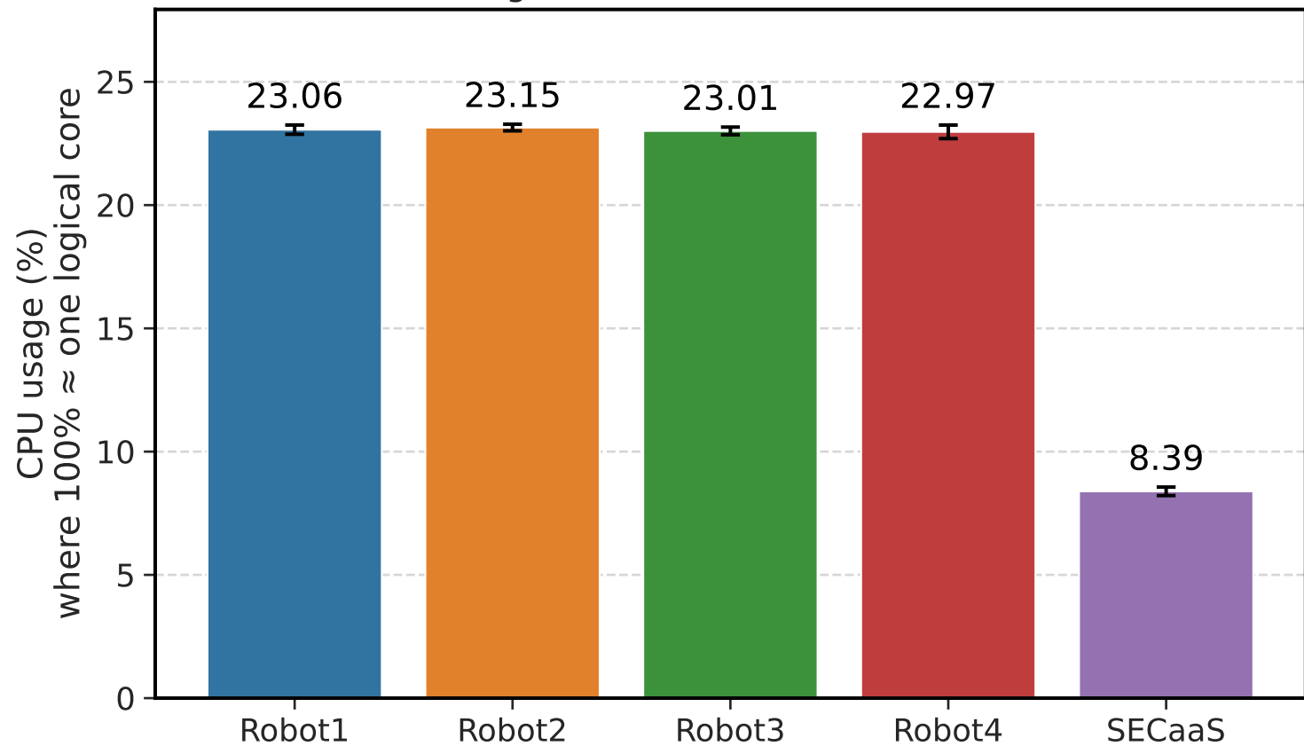
CPU usage of attestation-sidecar container
