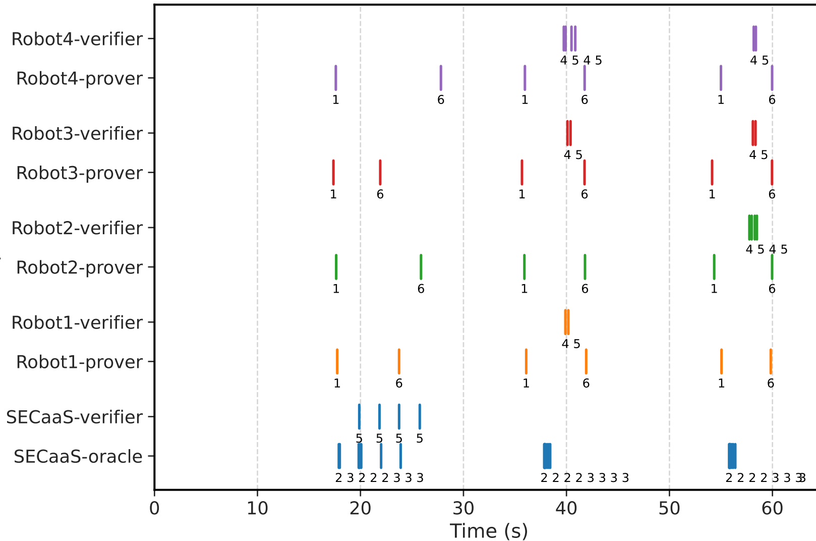
Attestation Event Flow (Run 1) - First 65s
