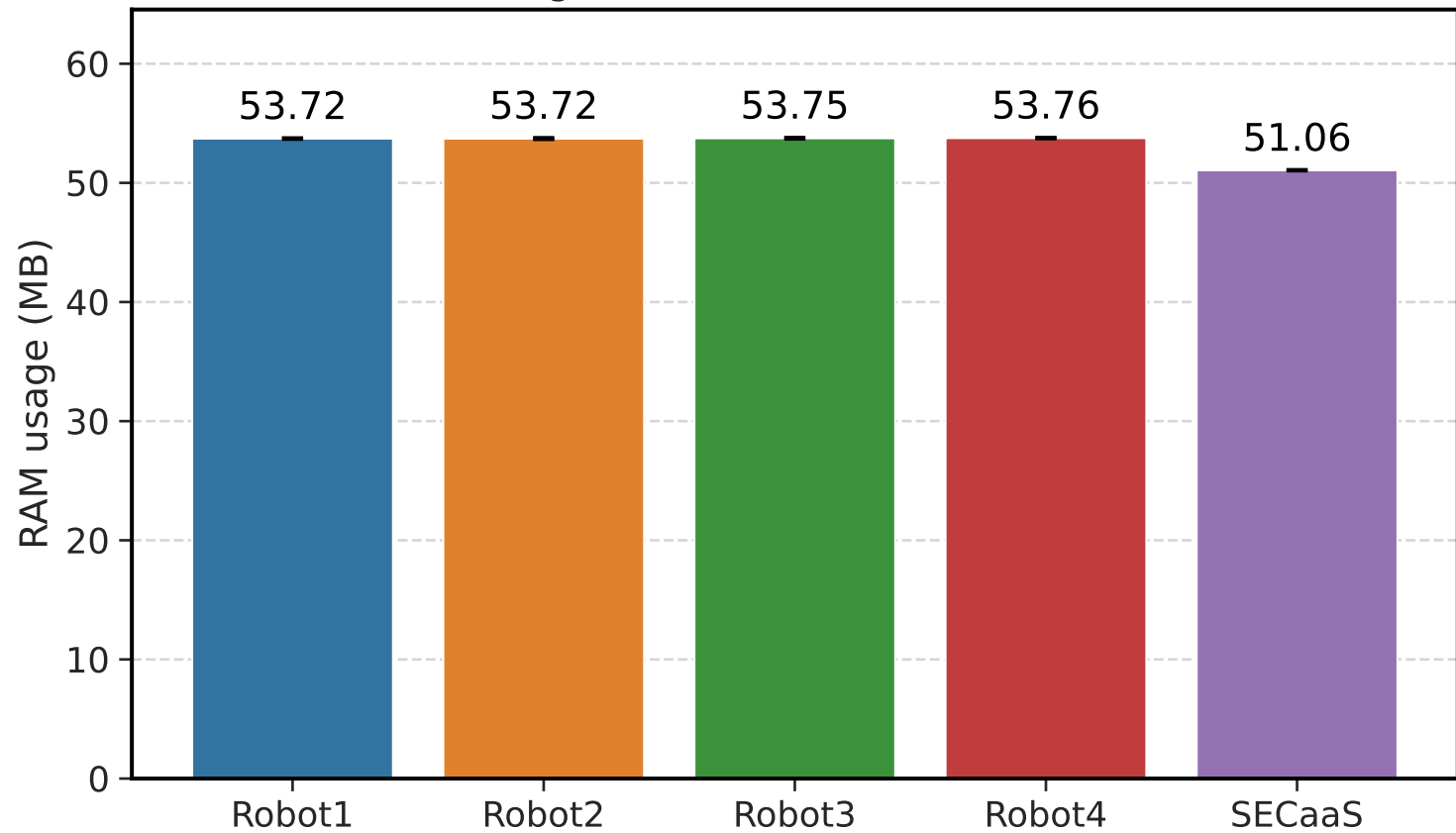
RAM usage of attestation-sidecar container
