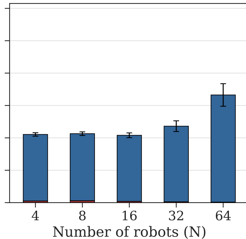
Continuous Attestation
