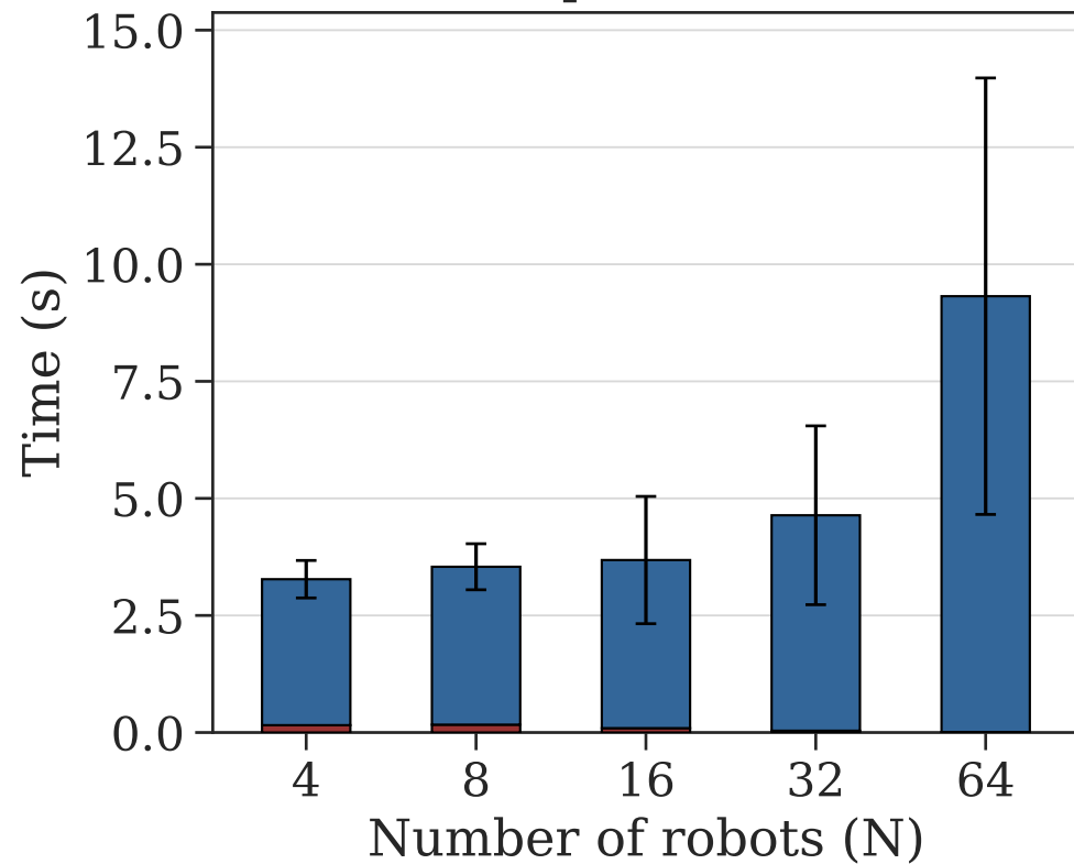
Startup Attestation
