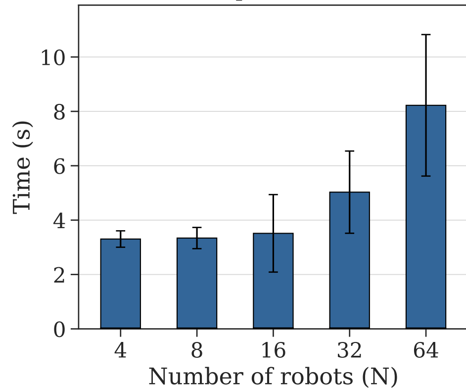
Startup Attestation
