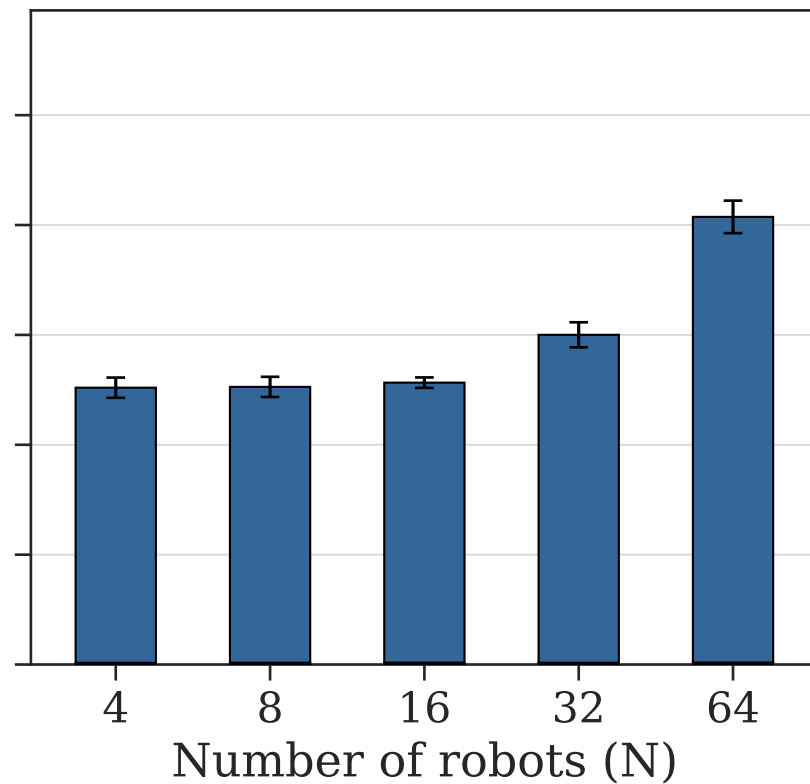
Continuous Attestation
