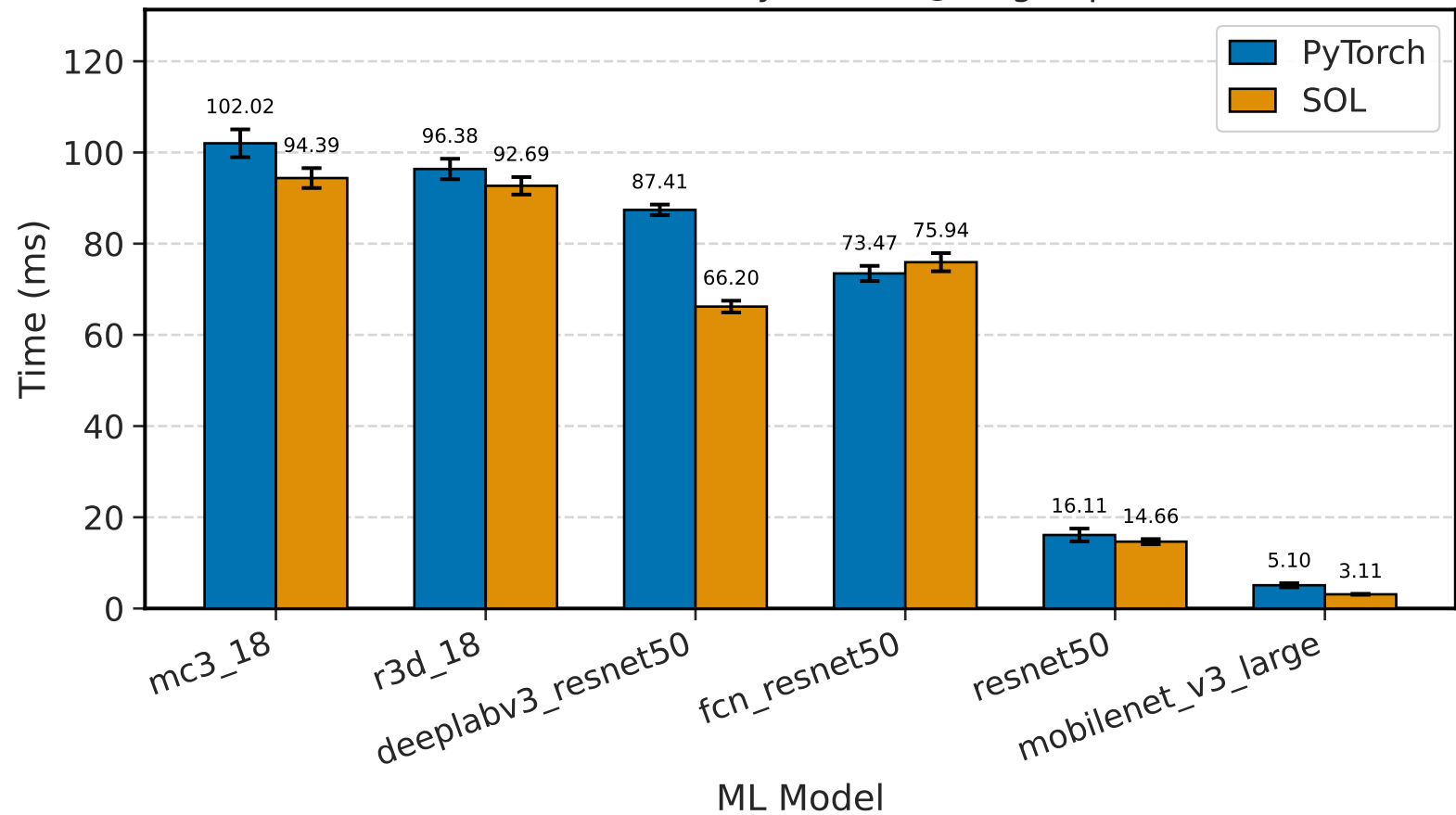
Inference latency - stock @ edge-cpu
