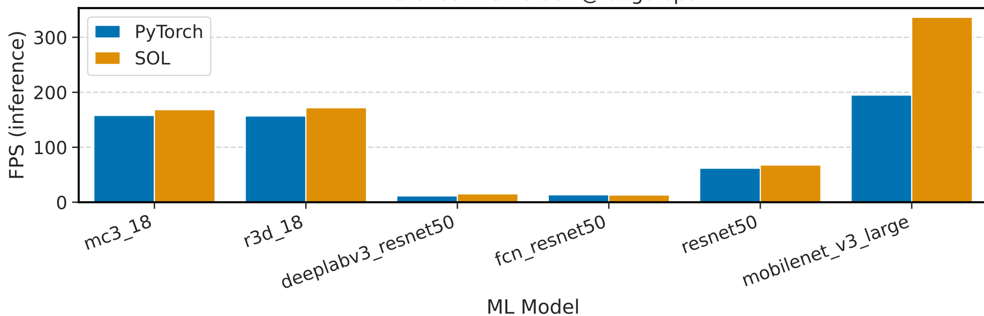
Inference FPS - stock @ edge-cpu
