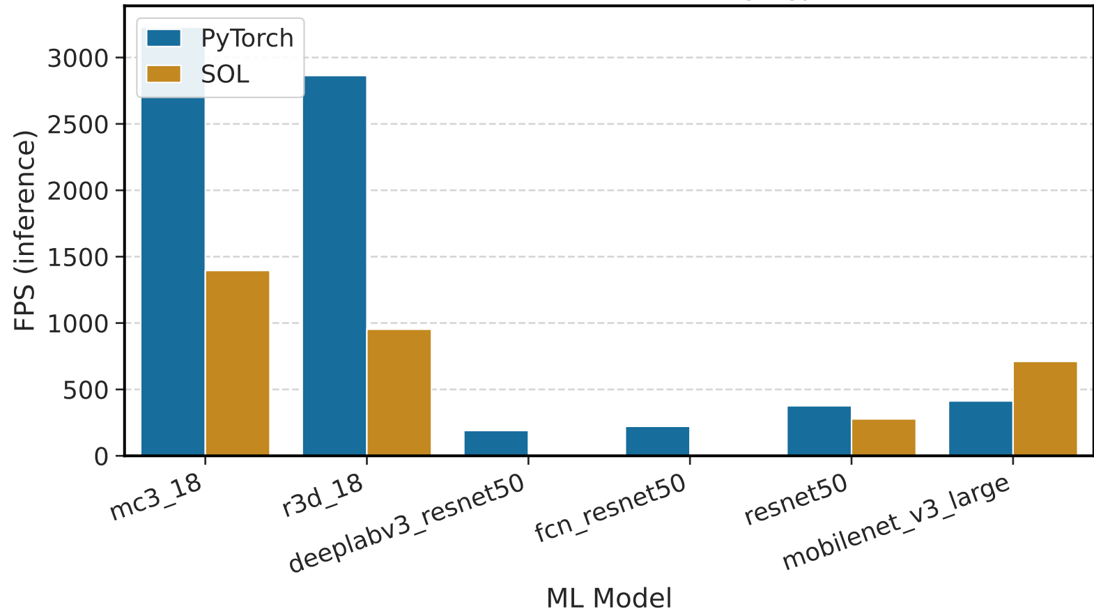
Inference FPS - stock @ edge-gpu
