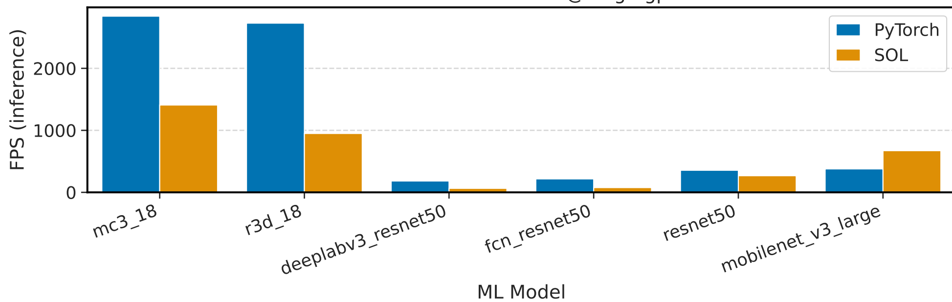
Inference FPS - stock @ edge-gpu
