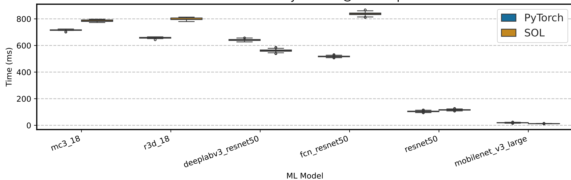
Inference latency - stock @ robot-cpu
