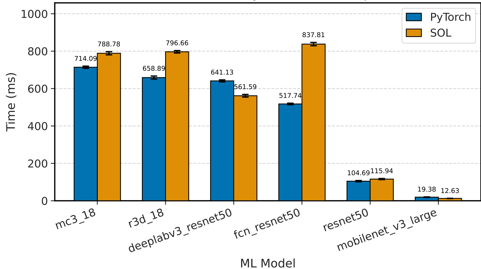
Inference latency - stock @ robot-cpu
