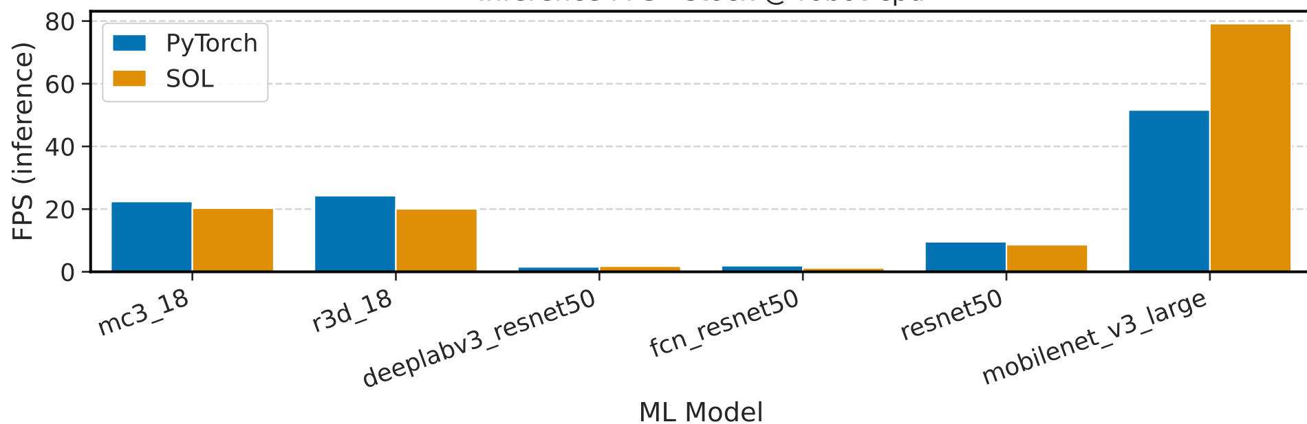
Inference FPS - stock @ robot-cpu
