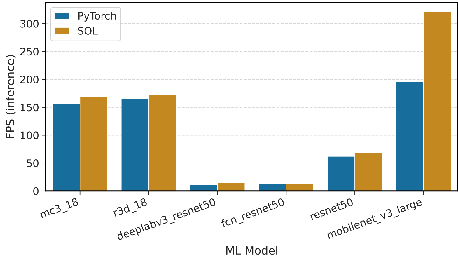
Inference FPS - stock @ edge-cpu
