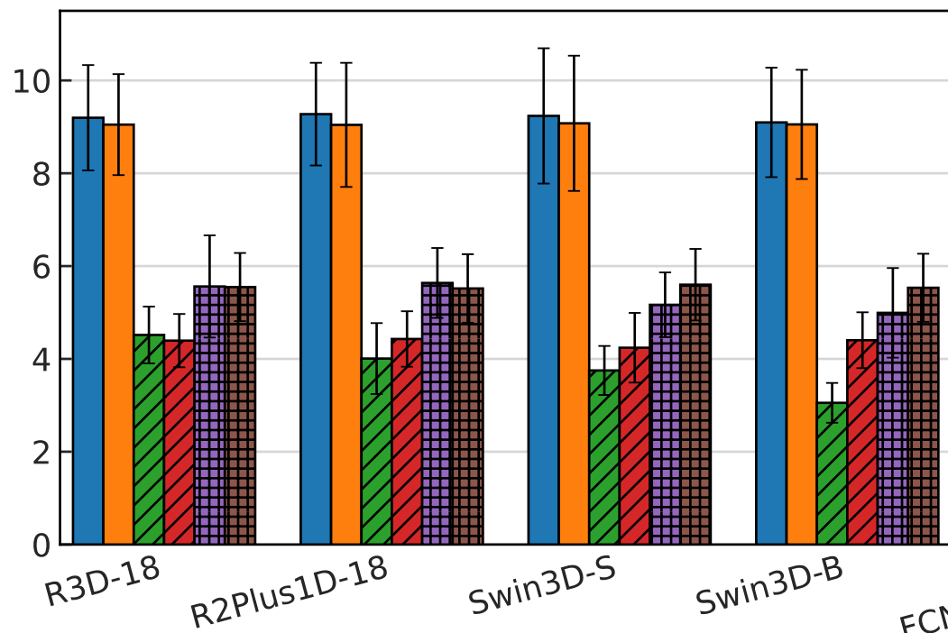
(b) Video Action Recognition
