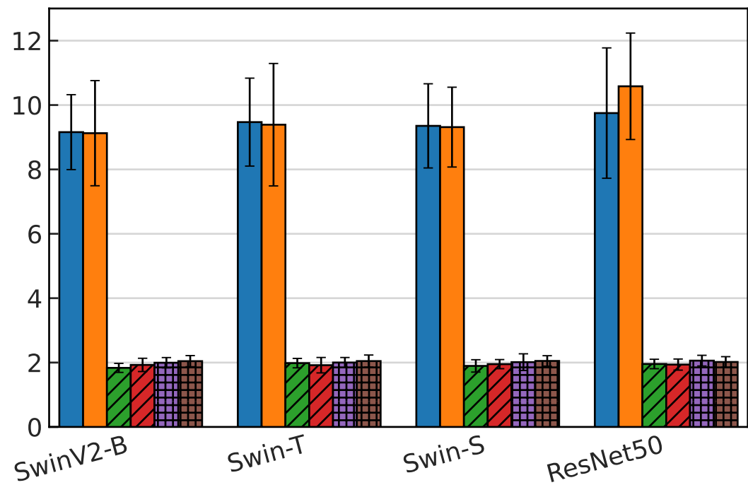
(a) Image Classification
