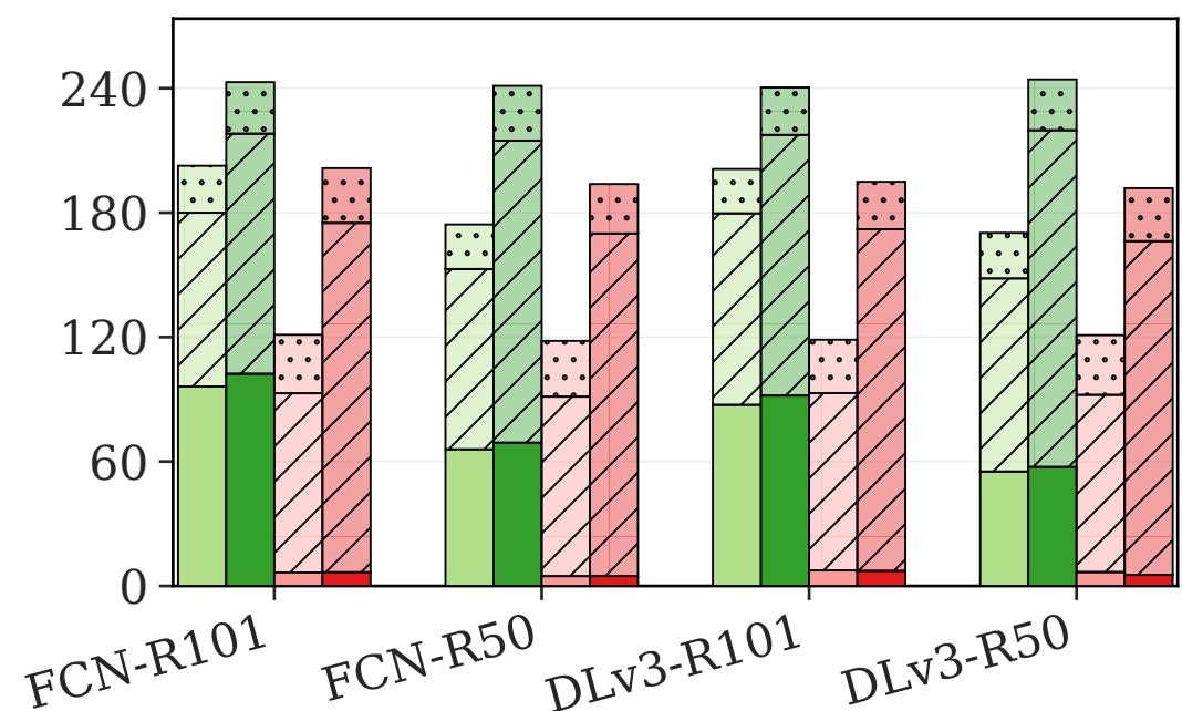
(c) Semantic Segmentation
