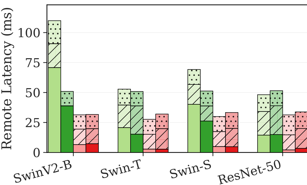
(a) Image Classification
