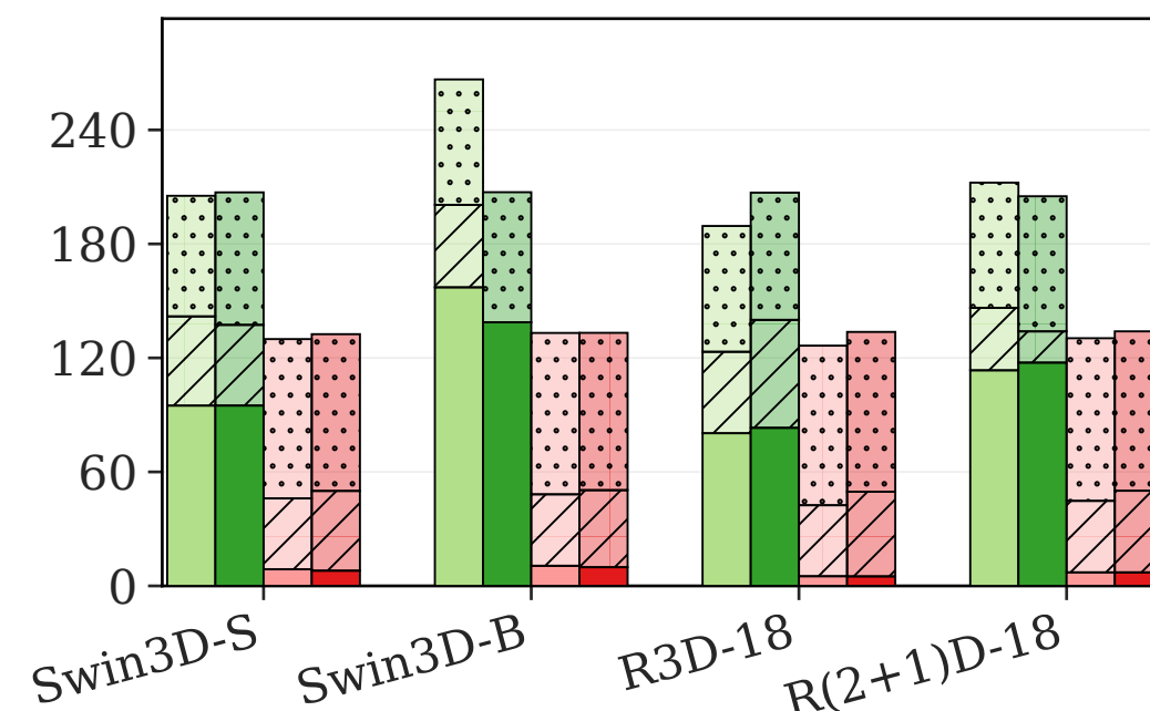
(b) Video Action Recognition
