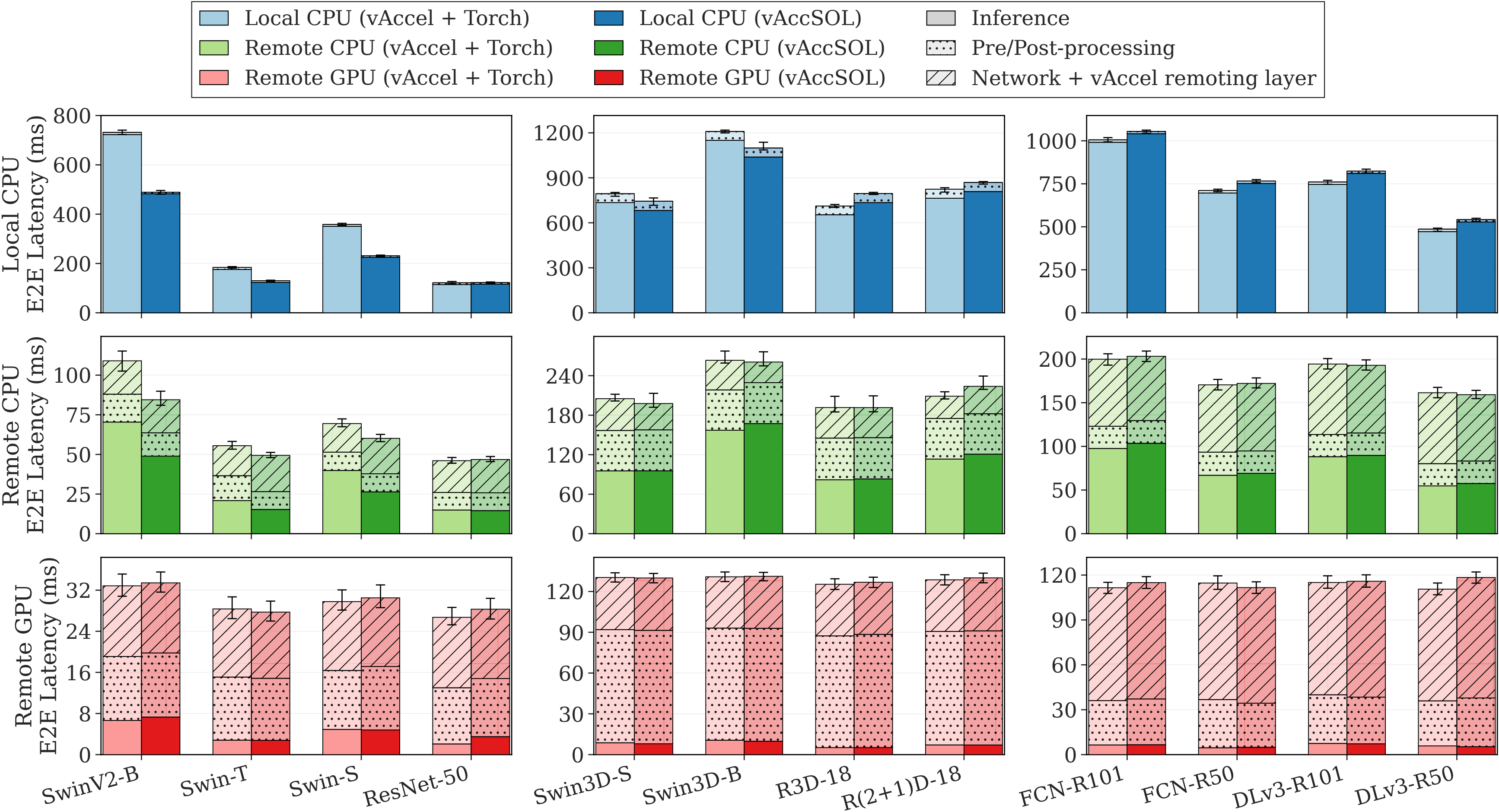
(a) Image Classification
