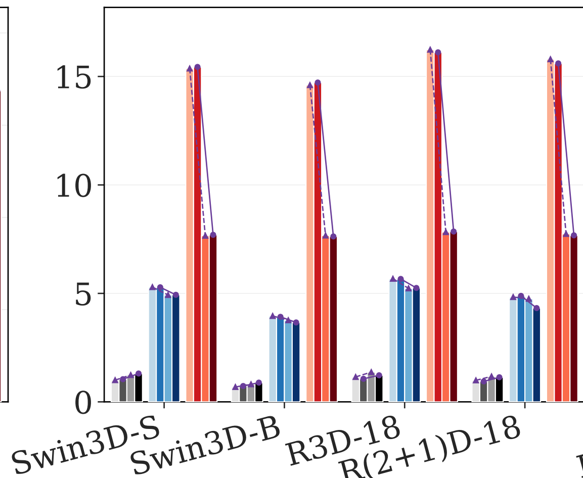
(b) Video Action Recognition
