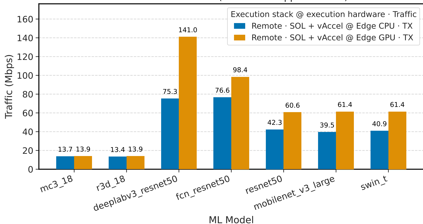
Robot network traffic (torchvision-app container)
