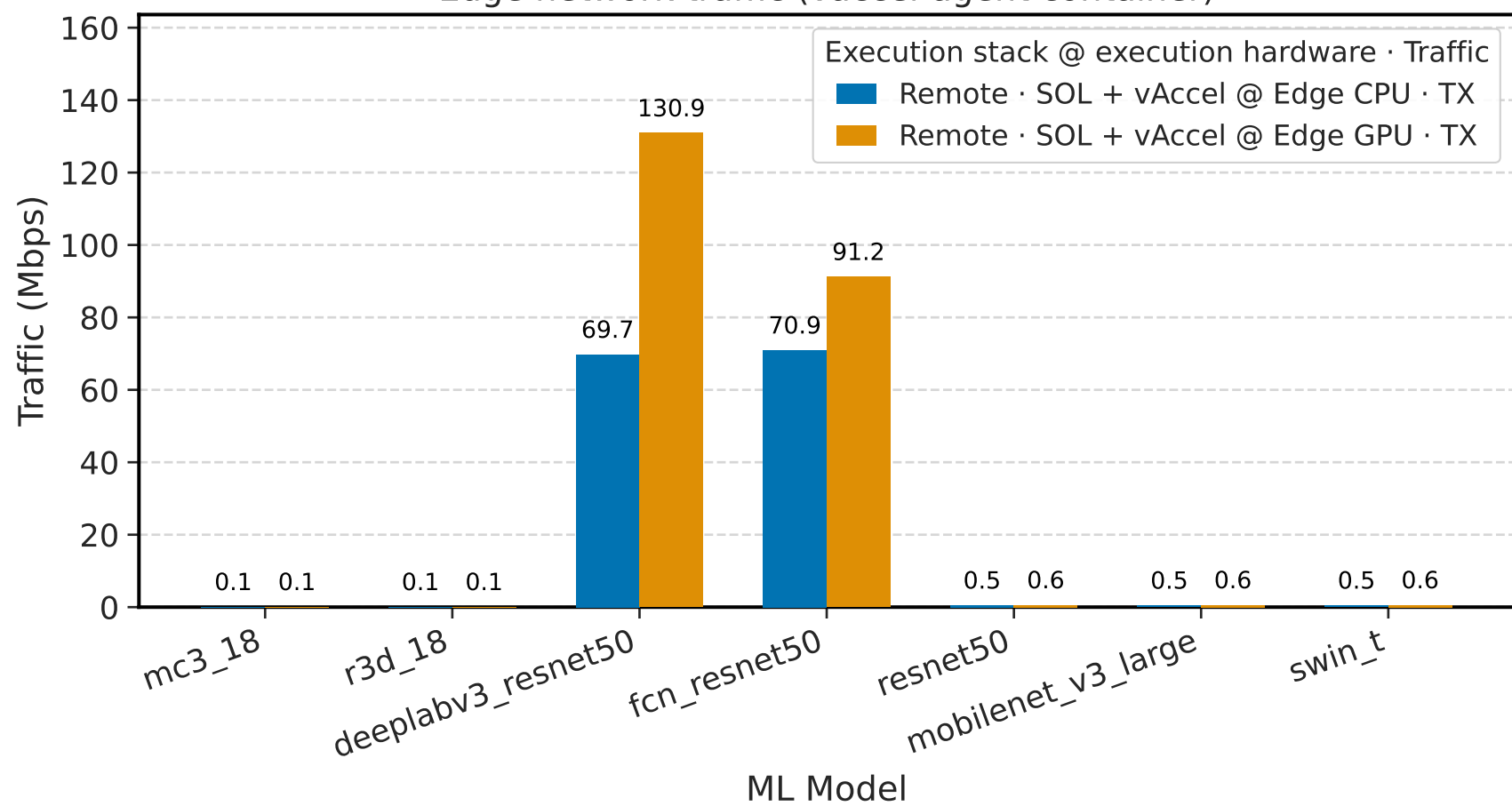
Edge network traffic (vaccel-agent container)
