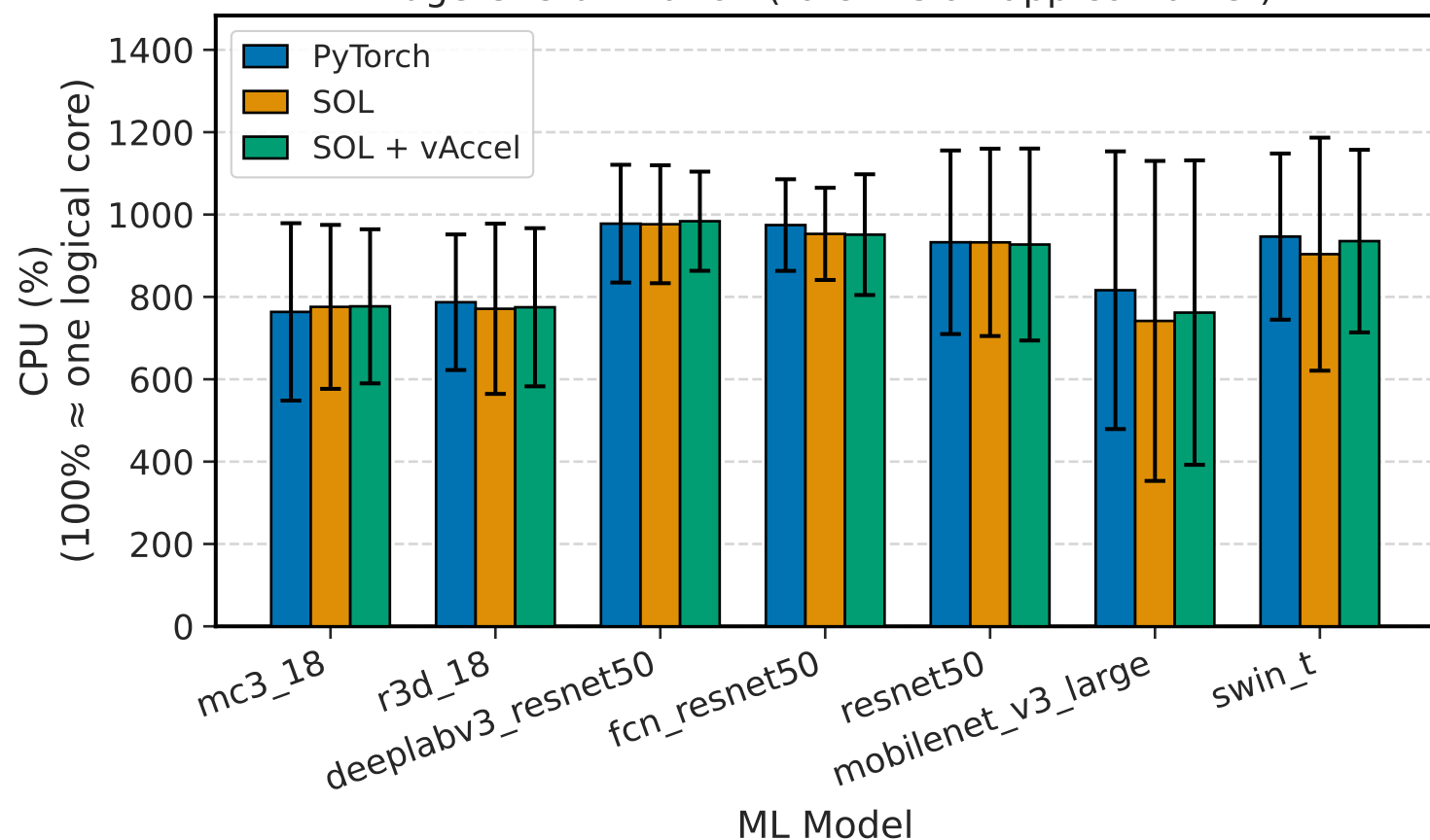
Edge CPU utilization (torchvision-app container)
