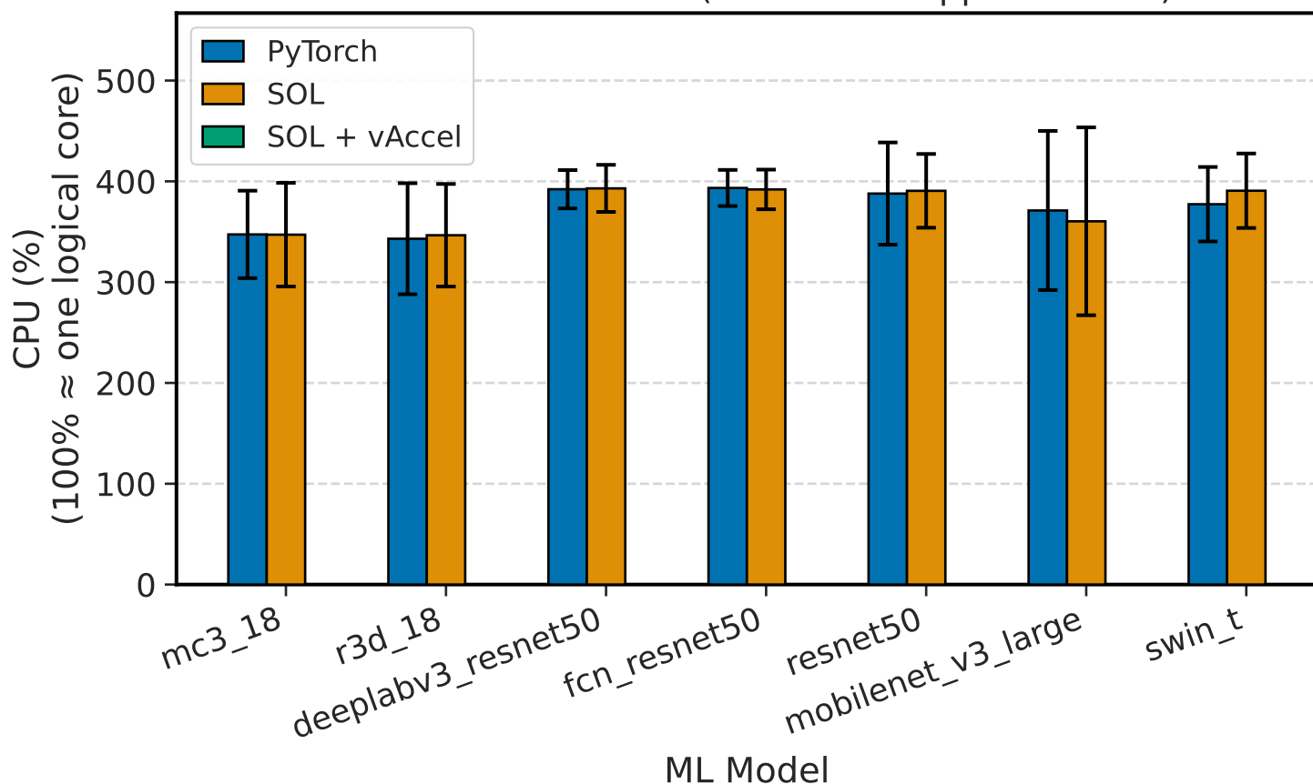
Robot CPU utilization (torchvision-app container)
