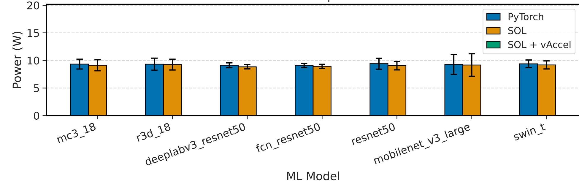
Robot CPU power
