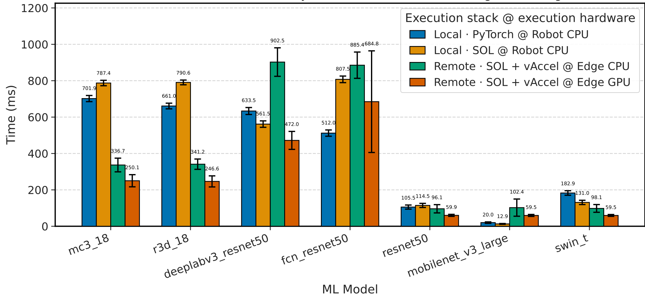
Robot-side inference latency under local execution and edge offloading
