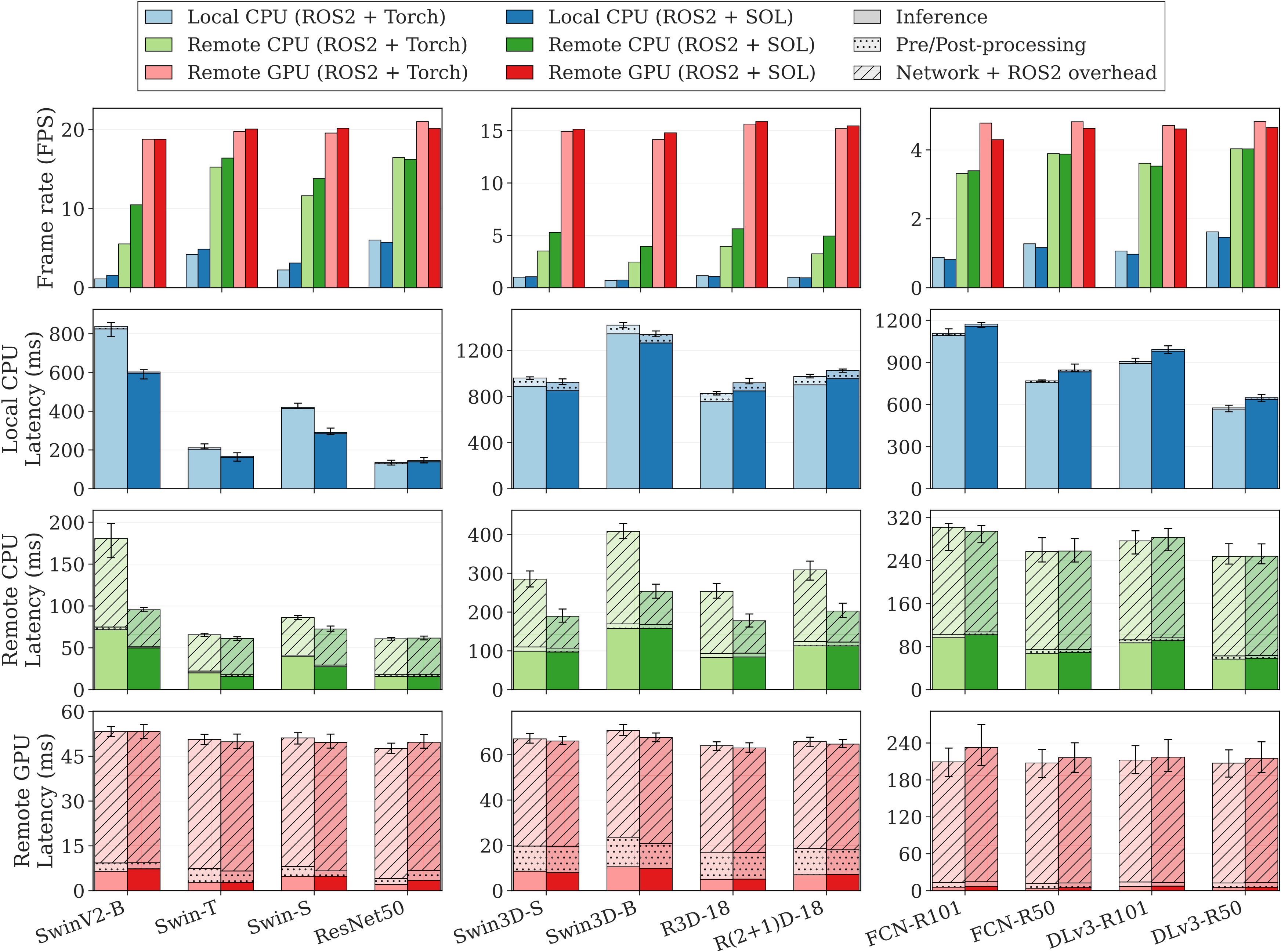
(a) Image Classification
