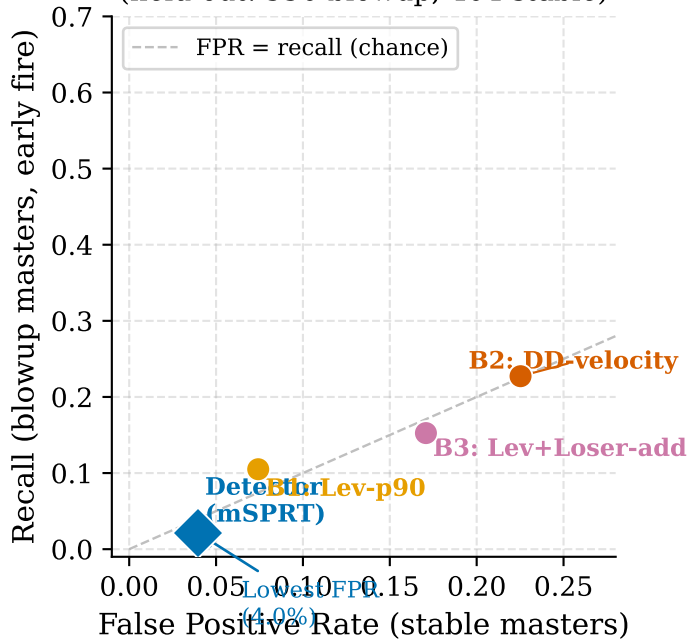
FPR / Recall trade-off (held-out: 990 blowup, 404 stable)
