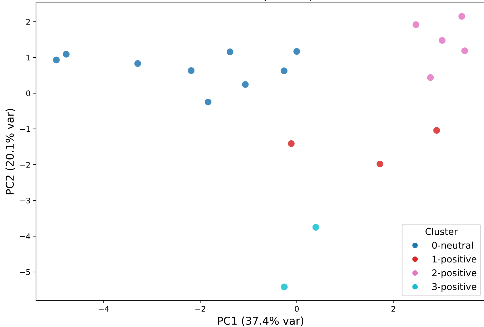
2D PCA of K-Means Clusters | k = 4 | Silhouette = 0.258
