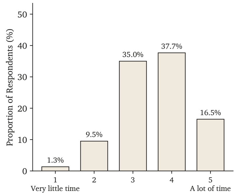
(c) Time Available for Research
