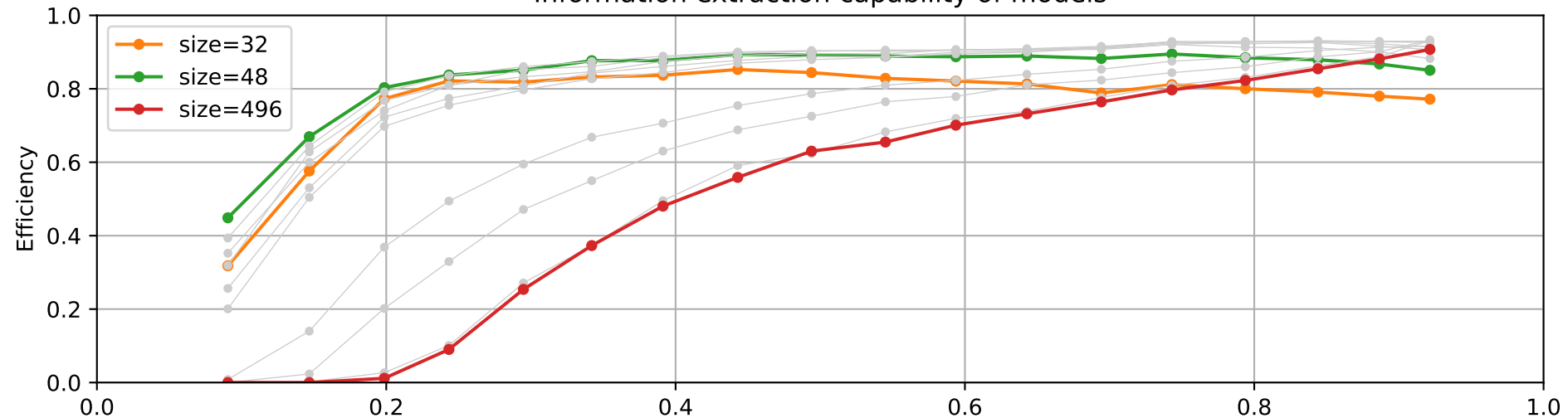
Information extraction capability of models
