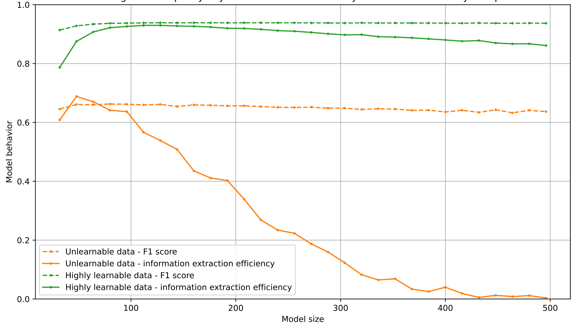
Scaling model capacity beyond a dataset's learnability limit creates a 'fidelity collapse'
