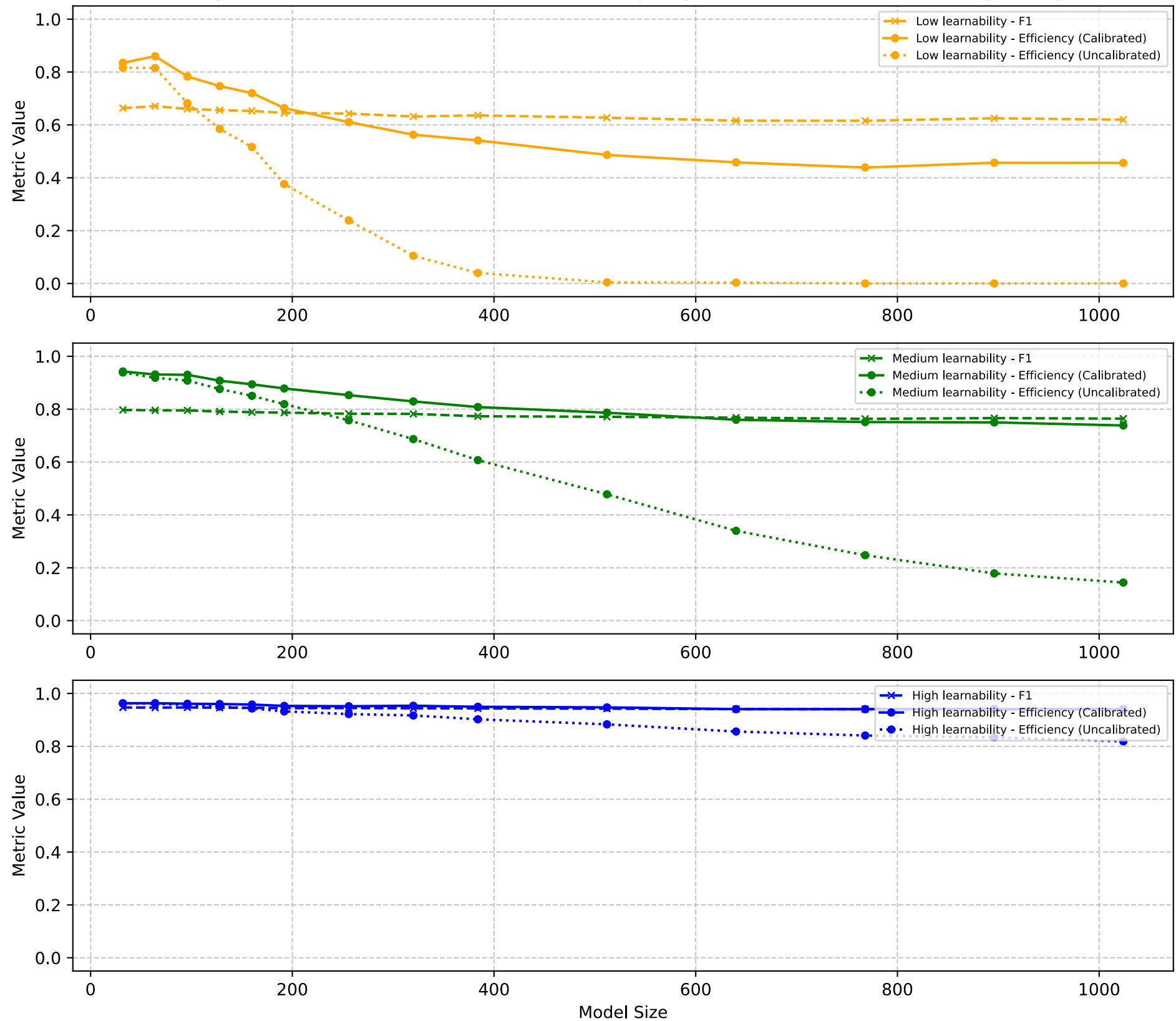
Accuracy remains stable while calibrated efficiency degrades with model size (low-signal regime)
