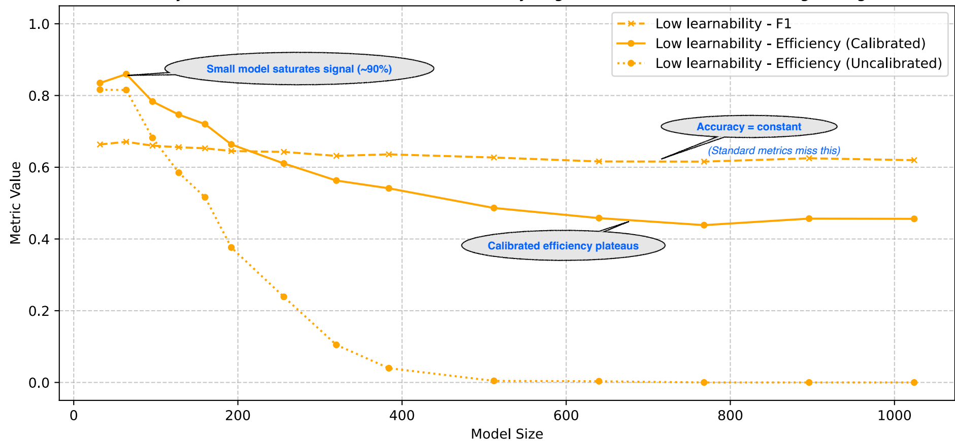
Accuracy remains stable while calibrated efficiency degrades with model size (low-signal regime)
