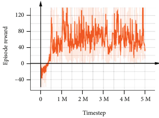
FIGURE 3: Episode reward.
