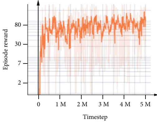
FIGURE 2: PPO2 episode.
