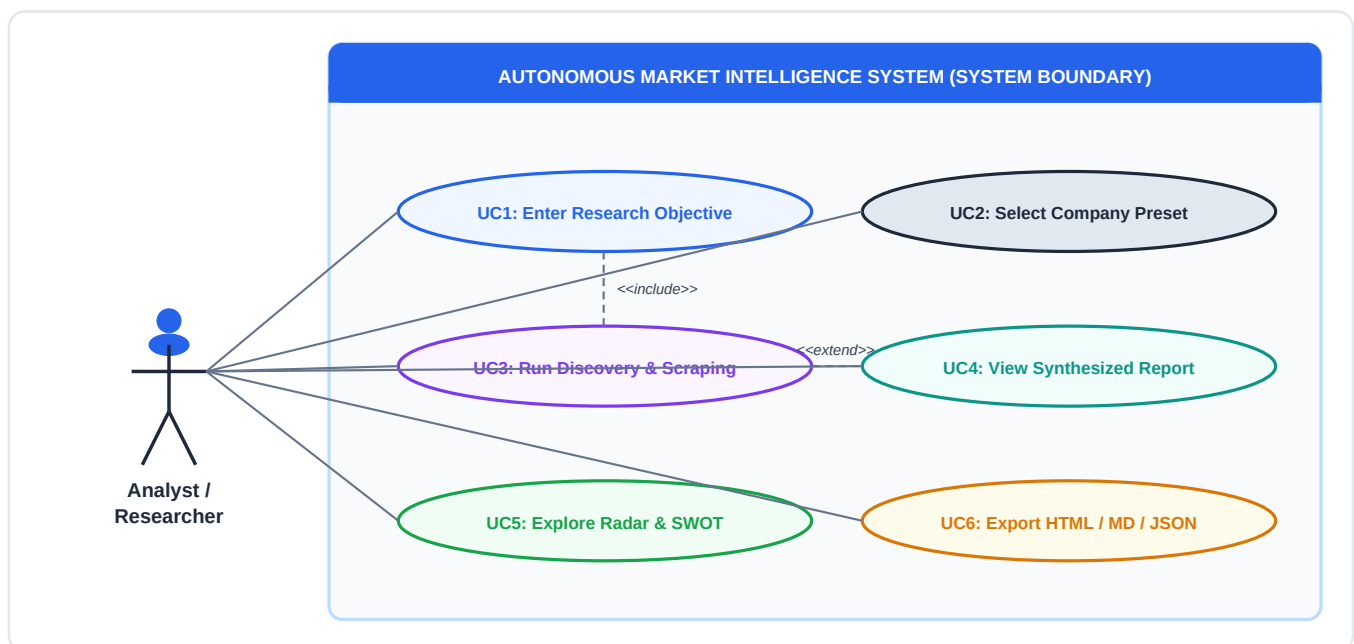
Figure 3. Use case diagram illustrating core analyst interactions, preset workflows, and automated pipeline execution
