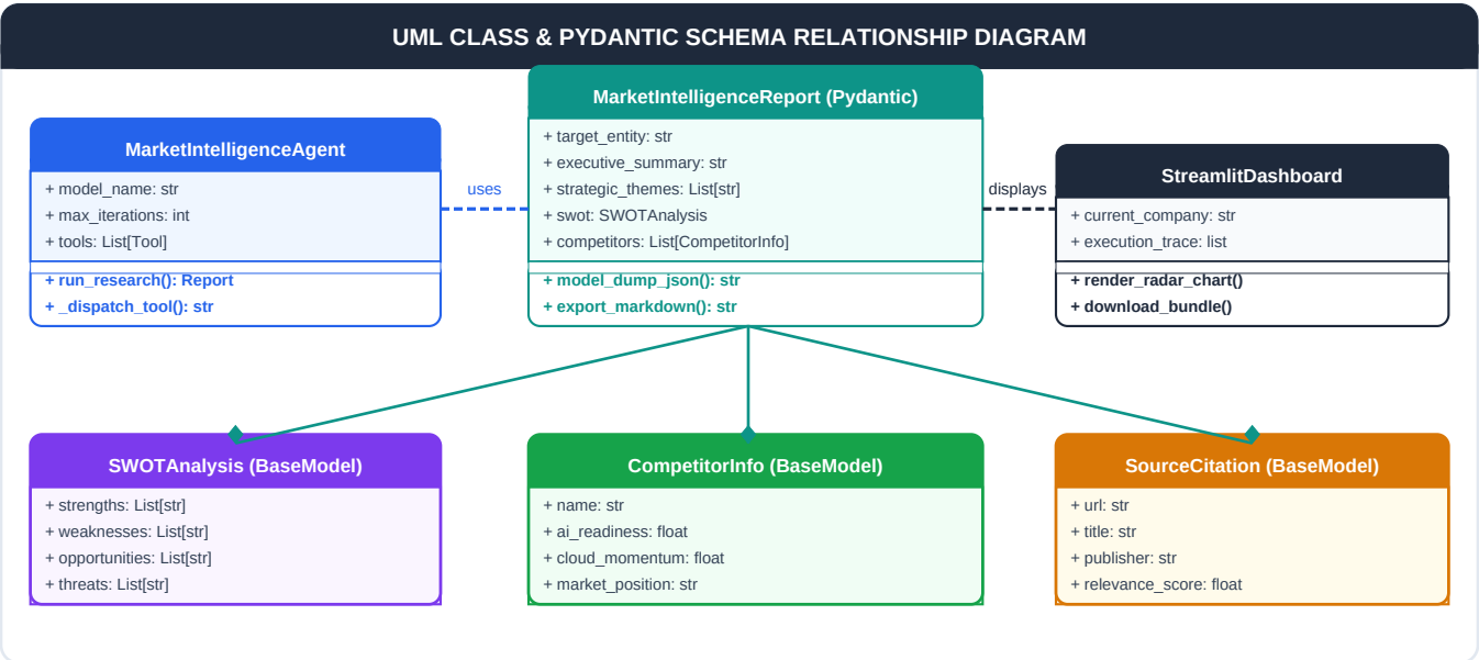
Figure 5. UML class and Pydantic v2 schema relationship diagram illustrating model composition and orchestration dependencies
