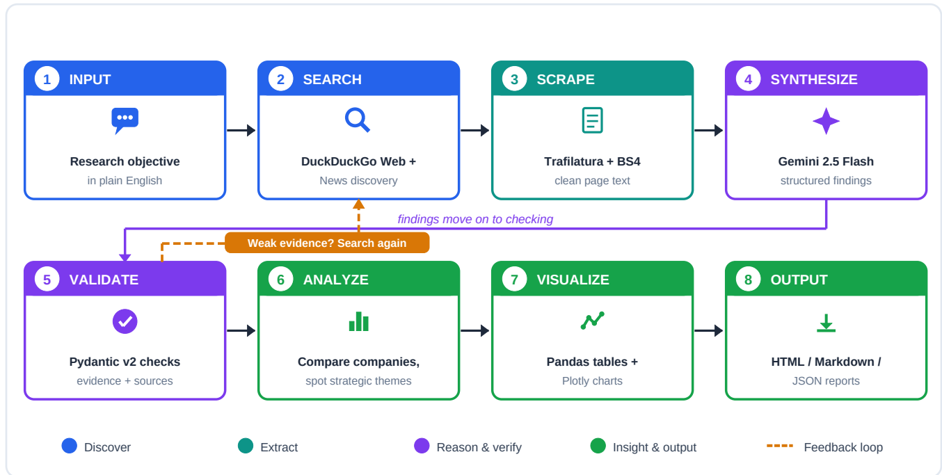
Figure 1. Agentic workflow / flow chart of the proposed system (8 stages, colour-coded by phase, with a feedback loop)
