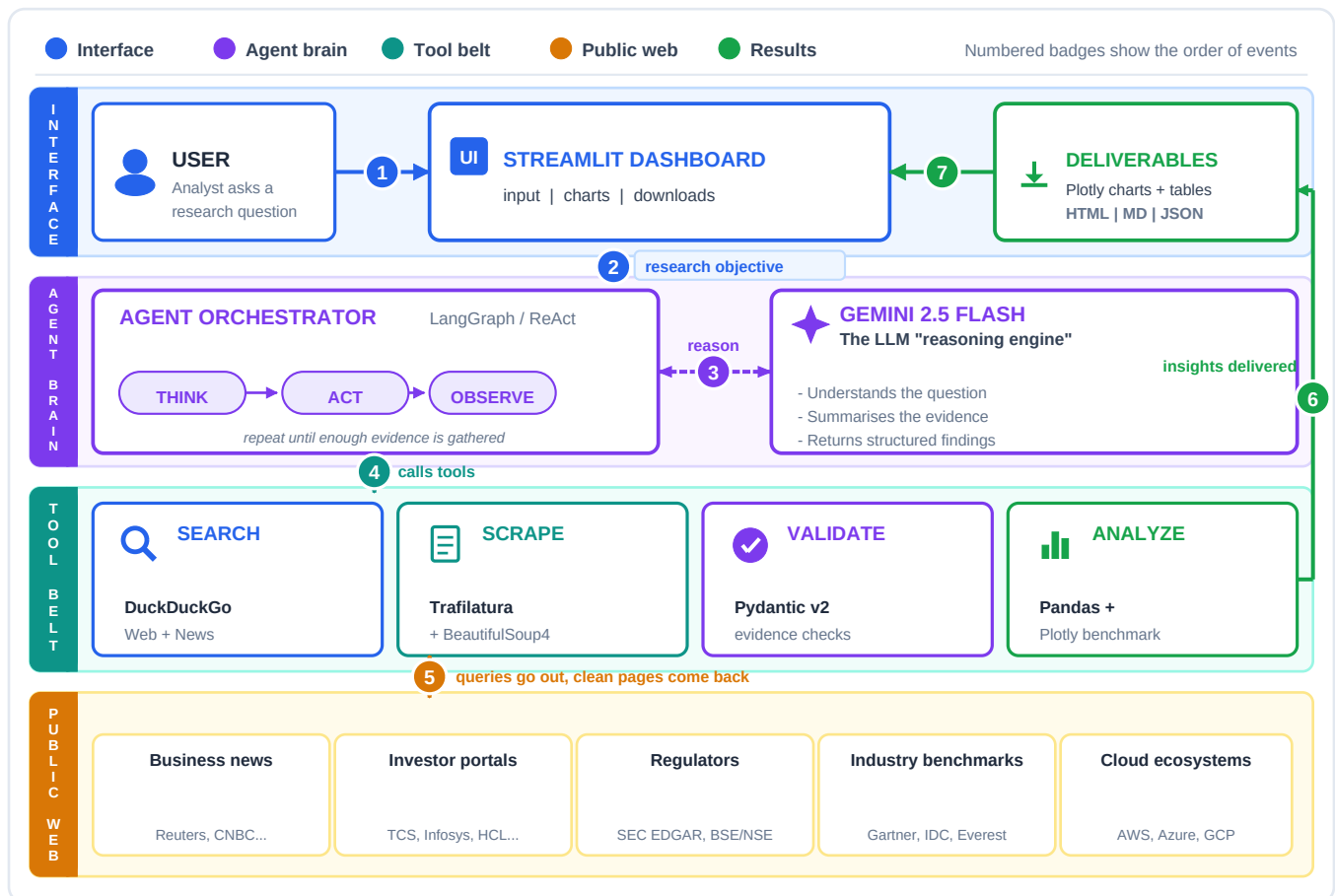
Figure 2. High-level system architecture (layered view: interface, agent brain, tool belt, public web, results)
