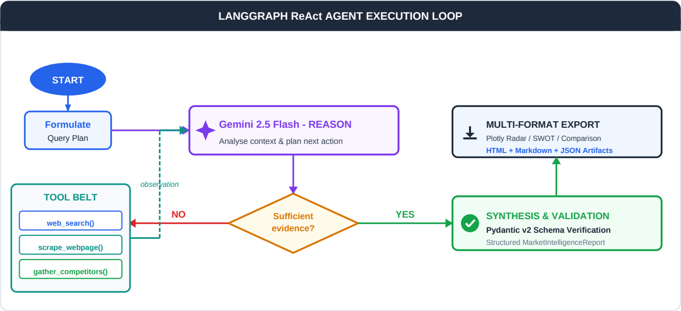
Figure 4. LangGraph ReAct agent state-machine and feedback loop execution model with tool dispatch and Pydantic validation
