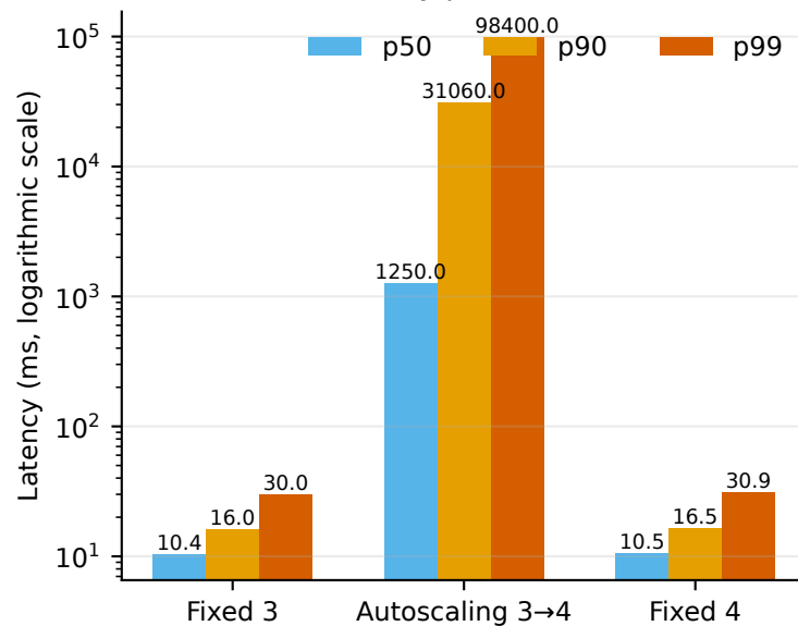
Latency percentiles
